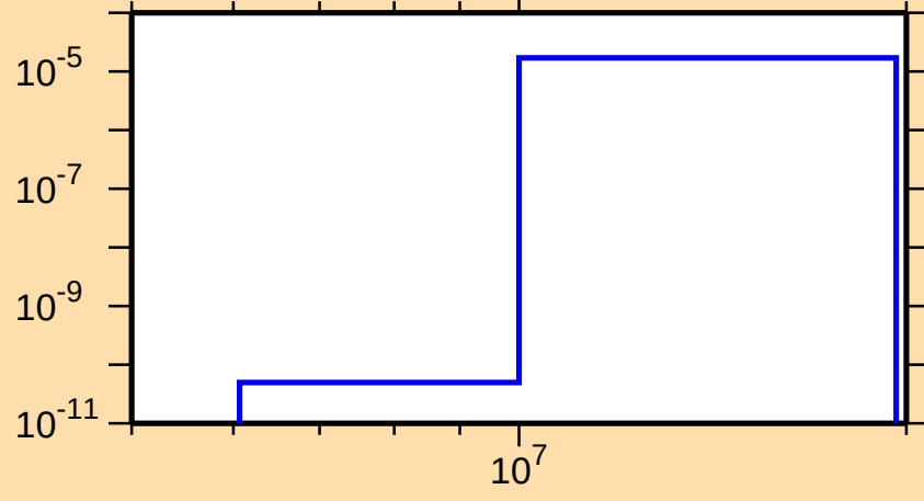
\sigma vs. E for ^{245}\text{Pu}(n,n\alpha)
