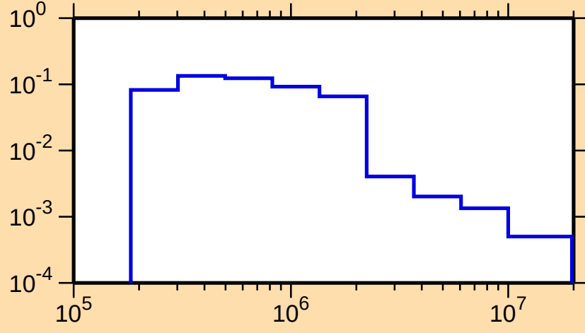
\sigma vs. E for ^{245}\text{Pu}(n,n_1)
