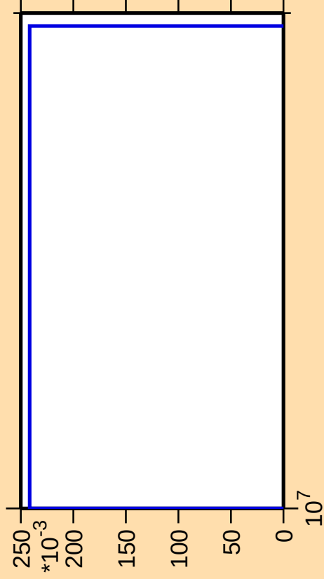
\Delta\sigma/\sigma vs. E for ^{245}\text{Pu}(n,\text{He3})
