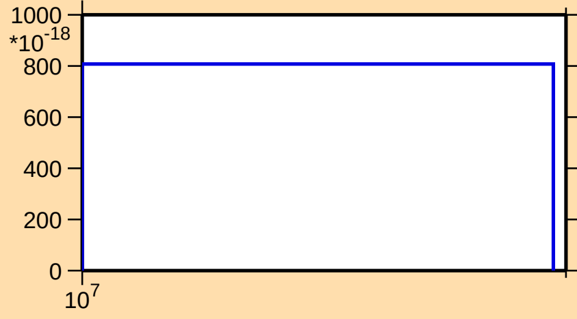
\sigma vs. E for ^{245}\text{Pu}(n,3n\alpha)
