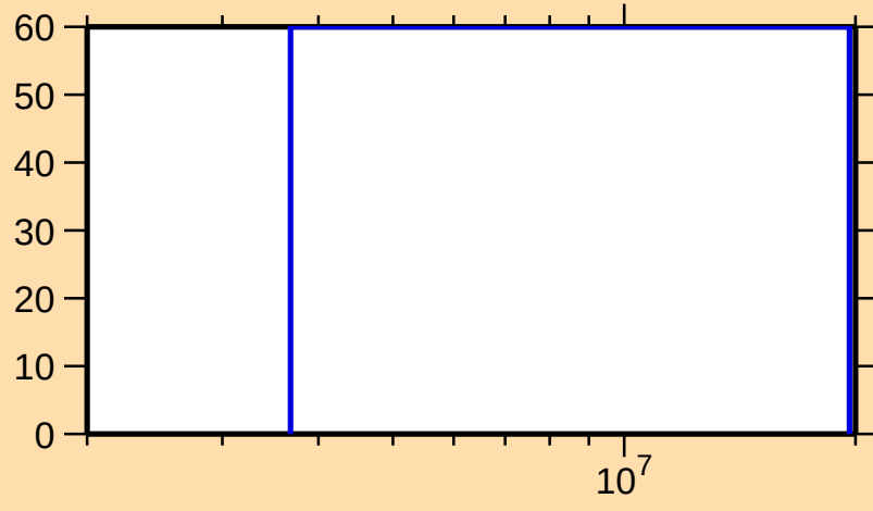
\Delta\sigma/\sigma vs. E for ^{245}\text{Pu}(n,2n)
