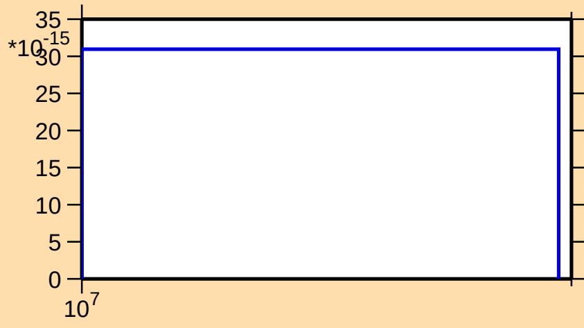
\sigma vs. E for ^{245}\text{Pu}(n,\text{He3})
