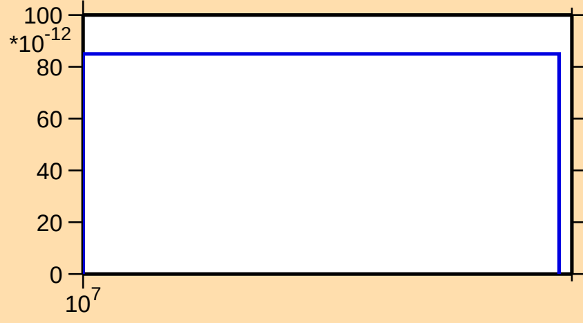
\sigma vs. E for ^{245}\text{Pu}(n,2np)
