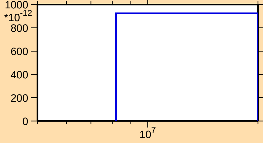
\sigma vs. E for ^{245}\text{Pu}(n,nt)
