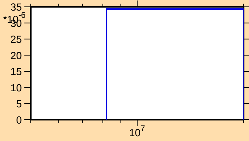
\sigma vs. E for ^{245}\text{Pu}(n,d)
