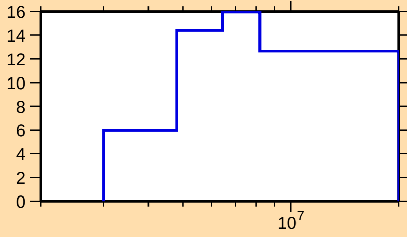
\Delta\sigma/\sigma vs. E for ^{245}\text{Pu}(n,\text{tot.})
