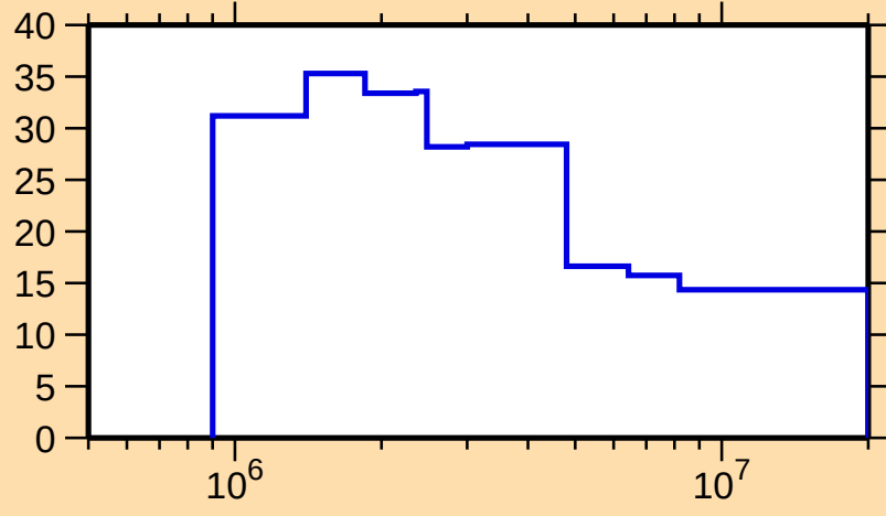
\Delta\sigma/\sigma vs. E for ^{245}\text{Pu}(n,\text{nonel.})
