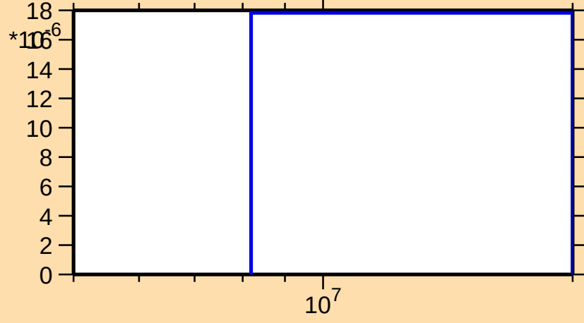
\sigma vs. E for ^{245}\text{Pu}(n,t)
