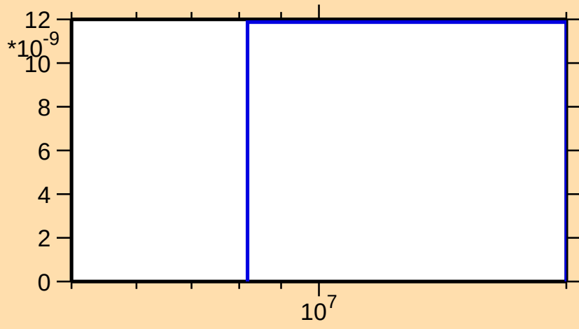
\sigma vs. E for ^{245}\text{Pu}(n,\text{nd})
