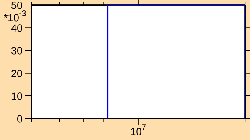
\sigma vs. E for ^{245}\text{Pu}(n,3n)
