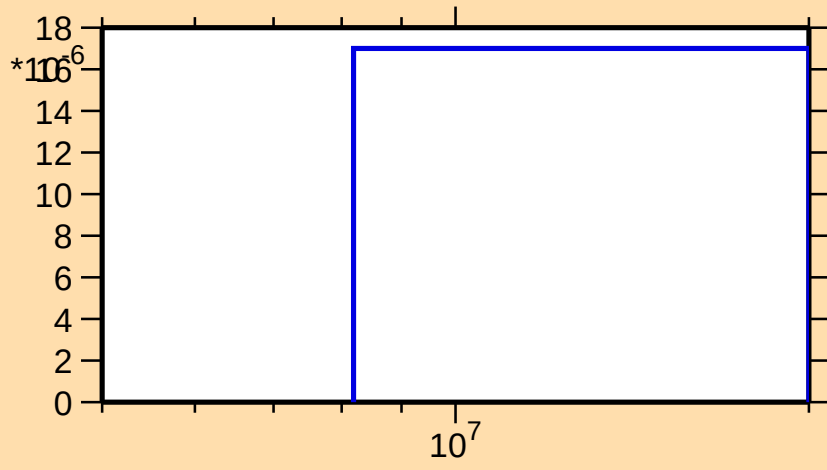
\sigma vs. E for ^{245}\text{Pu}(n,np)
