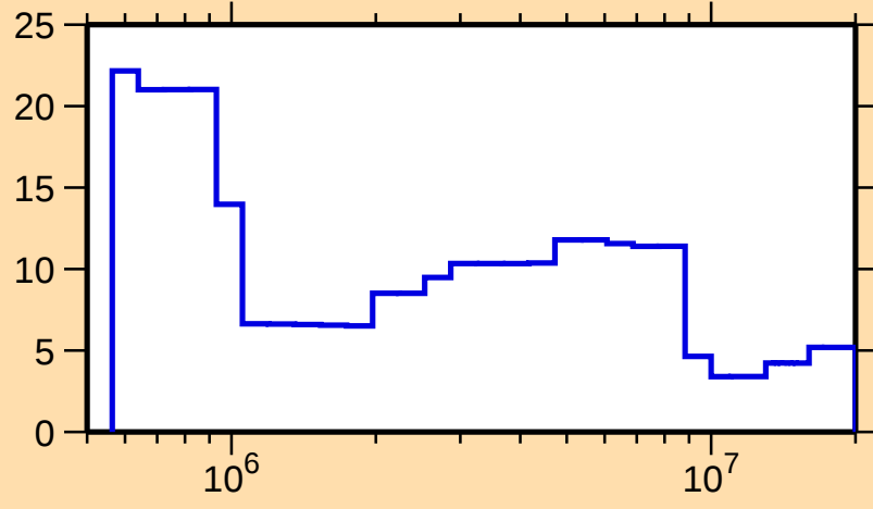
\Delta\sigma/\sigma vs. E for ^{212}\text{Ra}(n,\text{el.})
