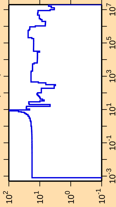
\Delta\sigma/\sigma vs. E for ^{212}\text{Ra}(n,\text{el.})
