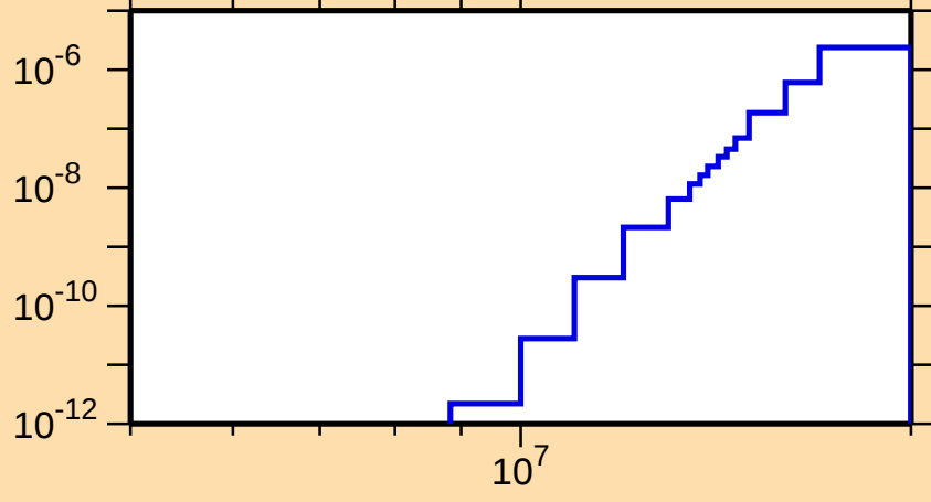
\sigma vs. E for ^{212}\text{Ra}(n,\text{He3})
