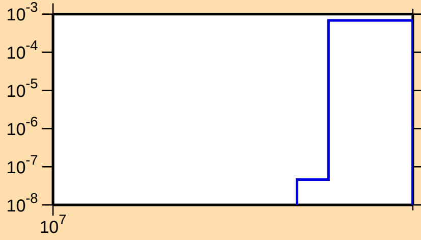
\sigma vs. E for ^{212}\text{Ra}(n,3n)
