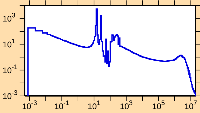
\sigma vs. E for ^{212}\text{Ra}(n,\gamma)
