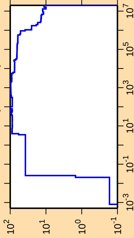
\Delta\sigma/\sigma vs. E for ^{212}\text{Ra}(n,\text{nonel.})
