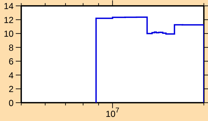
\Delta\sigma/\sigma vs. E for ^{212}\text{Ra}(n,\text{nonel.})
