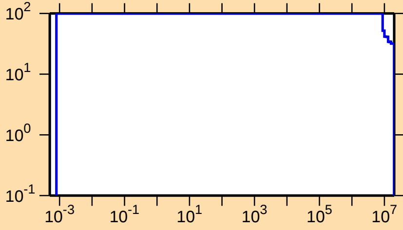
\Delta\sigma/\sigma vs. E for ^{212}\text{Ra}(n,p)
