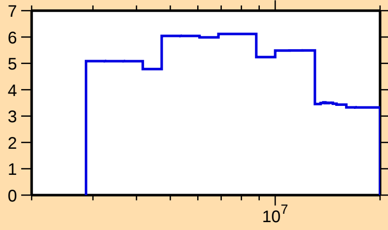
\Delta\sigma/\sigma vs. E for ^{212}\text{Ra}(n,\text{tot.})
