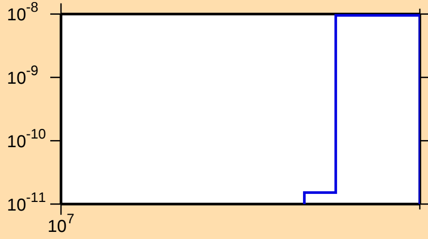
\sigma vs. E for ^{212}\text{Ra}(n,\text{nt})
