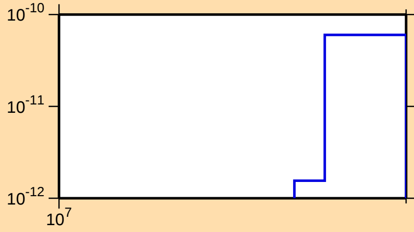
\sigma vs. E for ^{212}\text{Ra}(\text{mt } 34)
