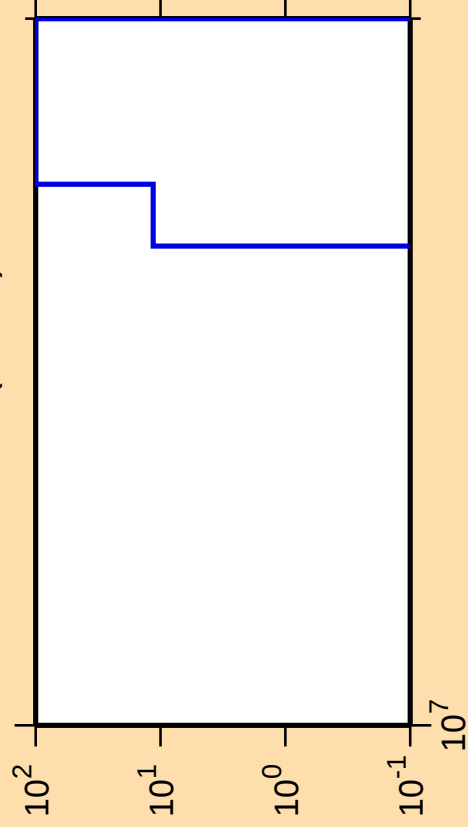
\Delta\sigma/\sigma vs. E for ^{212}\text{Ra}(\text{mt } 34)
