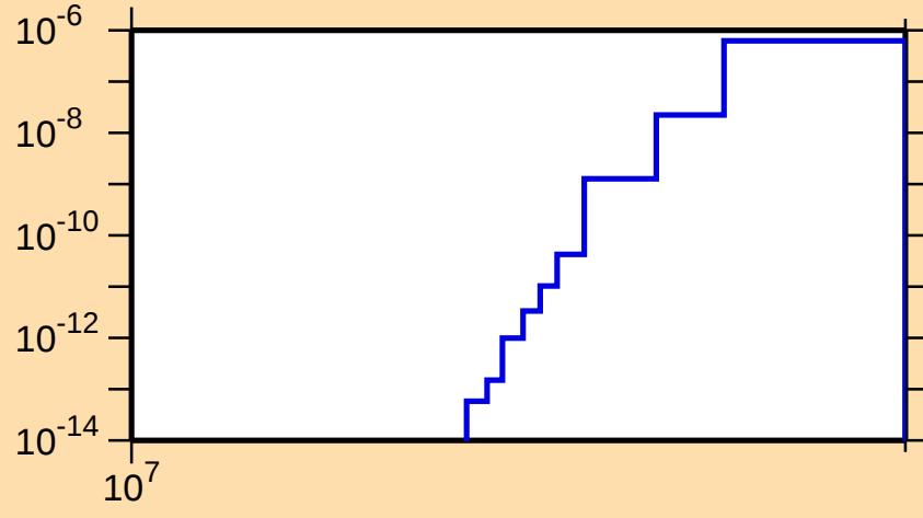
\sigma vs. E for ^{212}\text{Ra}(n,\text{nd})
