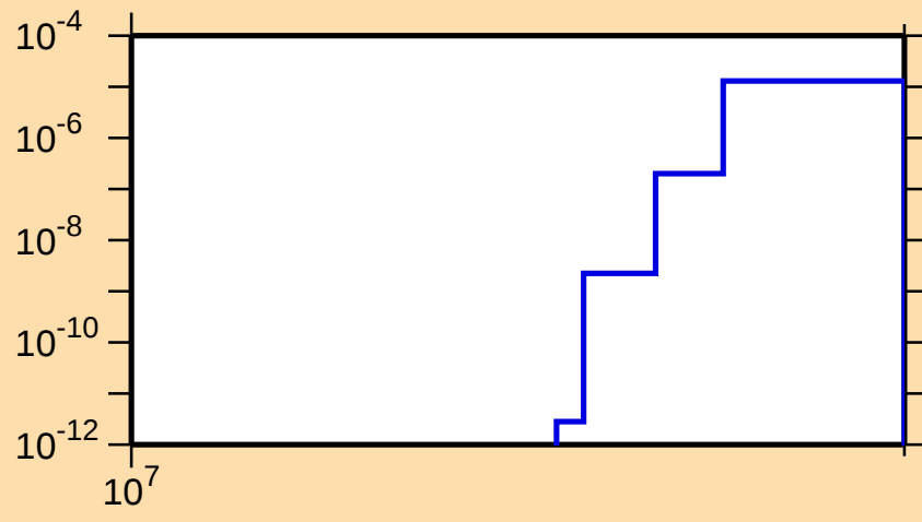
\sigma vs. E for ^{212}\text{Ra}(n,2np)
