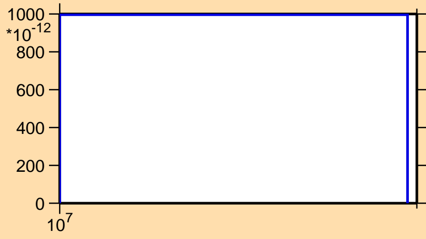
\sigma vs. E for ^{212}\text{Ra}(\text{mt117})
