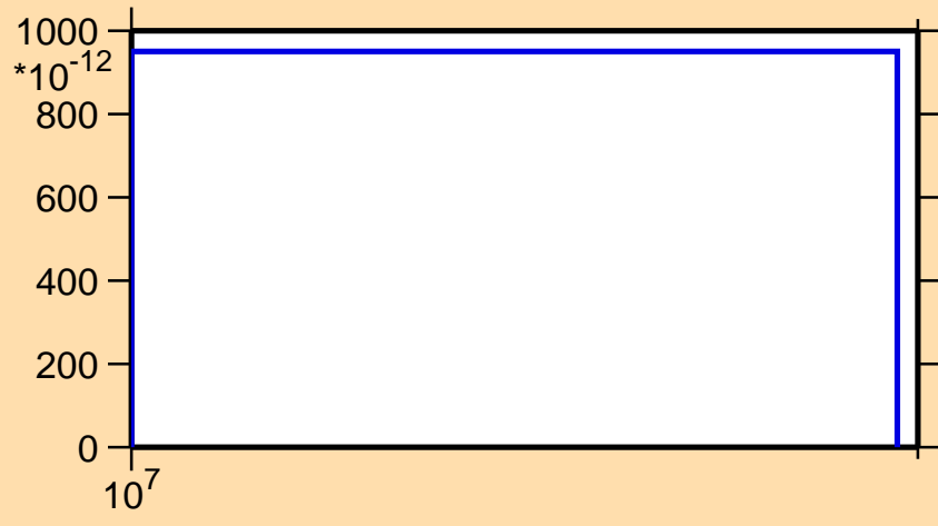
\sigma vs. E for ^{212}\text{Ra}(n,\text{pd})
