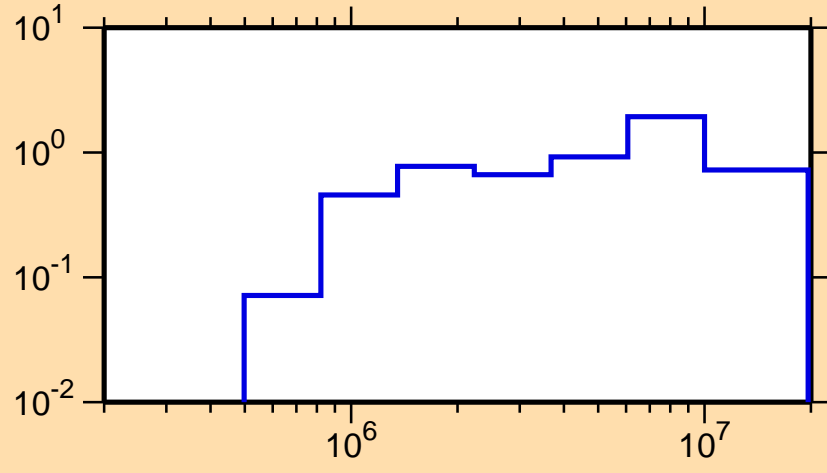
\sigma vs. E for ^{212}\text{Ra}(n,\text{inel.})
