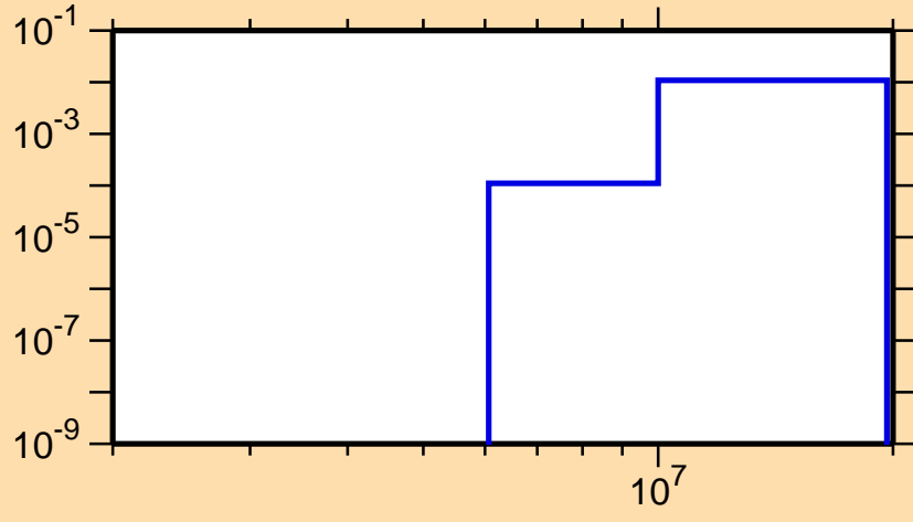
\sigma vs. E for ^{212}\text{Ra}(n,np)
