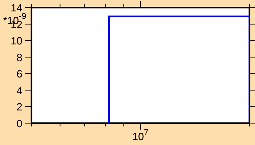
\sigma vs. E for ^{212}\text{Ra}(n,3n\alpha)
