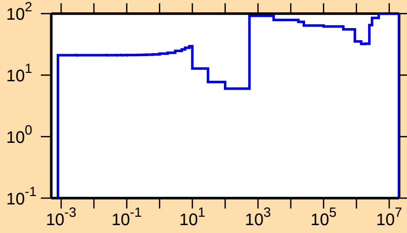
\Delta\sigma/\sigma vs. E for ^{212}\text{Ra}(n,\gamma)
