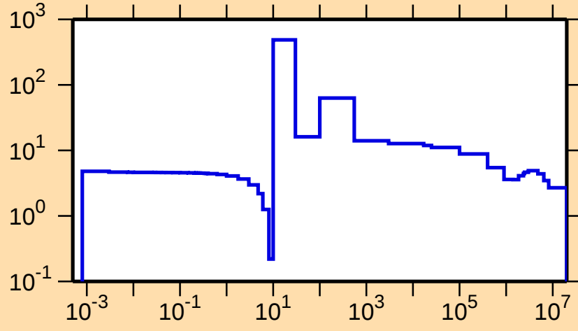
\sigma vs. E for ^{212}\text{Ra}(n,\text{el.})
