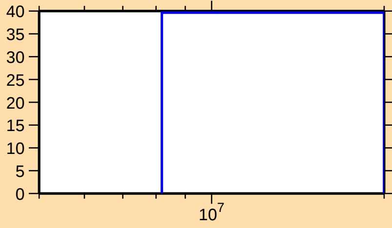
\Delta\sigma/\sigma vs. E for ^{212}\text{Ra}(n,2n)
