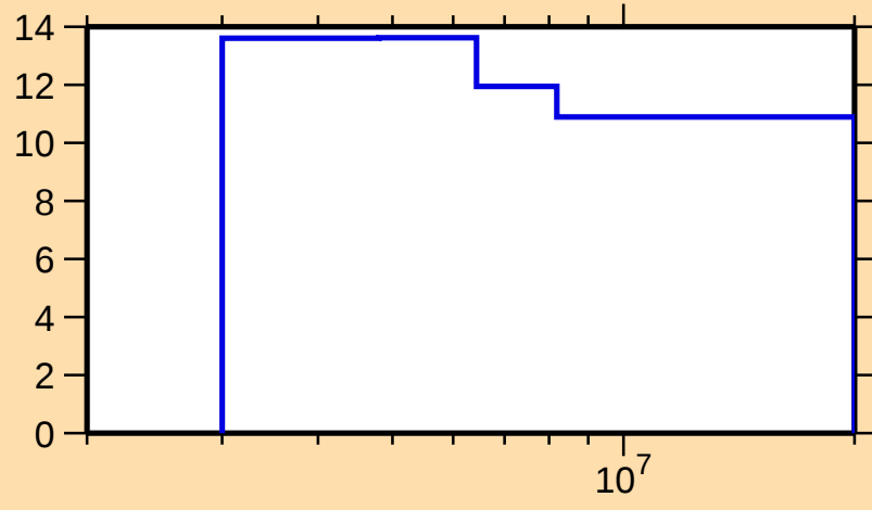
\Delta\sigma/\sigma vs. E for ^{212}\text{Ra}(n,n\text{onel.})
