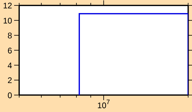
\Delta\sigma/\sigma vs. E for ^{212}\text{Ra}(n,\text{nonel.})
