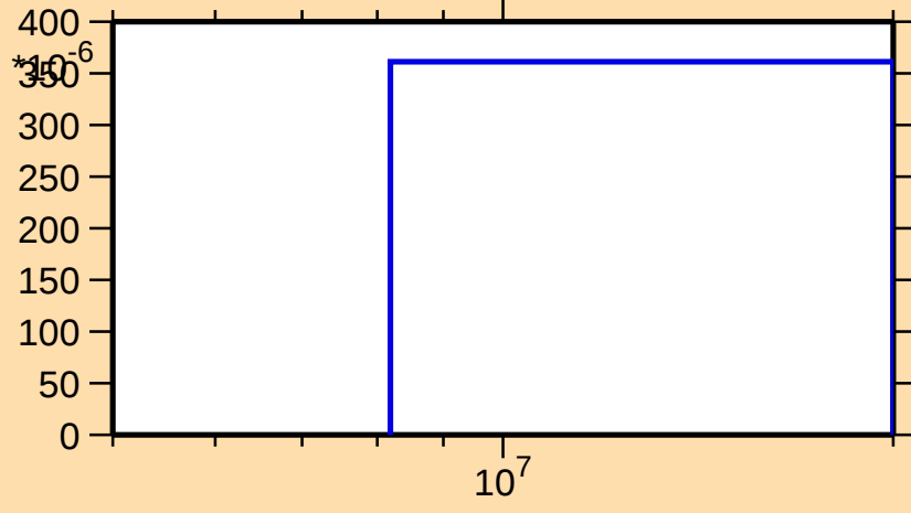
\sigma vs. E for ^{212}\text{Ra}(n,2n\alpha)
