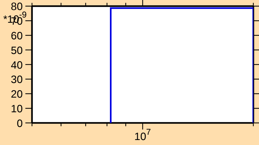
\sigma vs. E for ^{212}\text{Ra}(n,\text{He}3)
