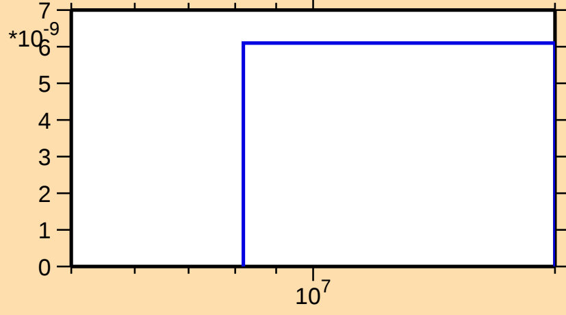
\sigma vs. E for ^{212}\text{Ra}(n,\text{nd})
