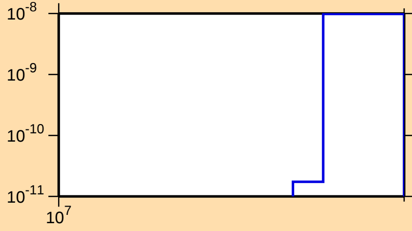
\sigma vs. E for ^{213}\text{Ra}(n,\text{nt})
