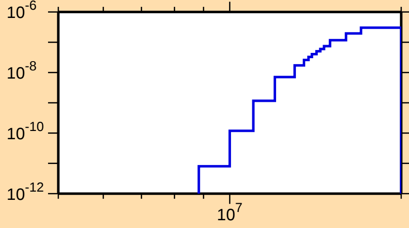
\sigma vs. E for ^{213}\text{Ra}(\text{mt117})
