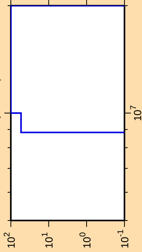
\Delta\sigma/\sigma vs. E for ^{213}\text{Ra}(\text{mt117})
