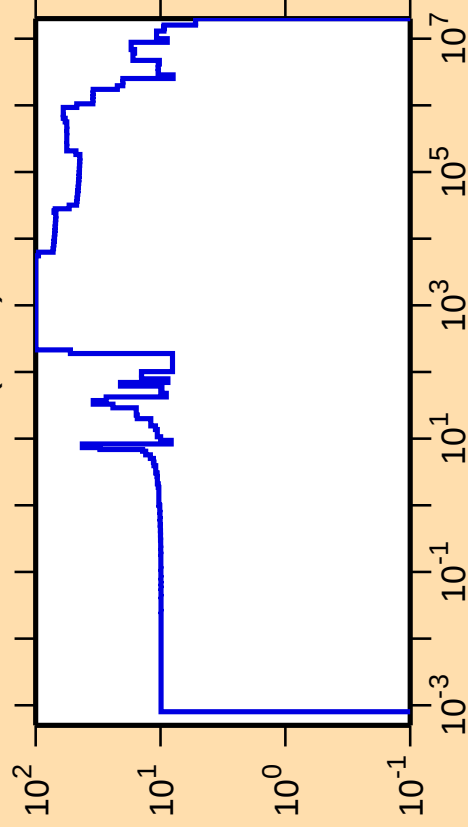
\Delta\sigma/\sigma vs. E for ^{213}\text{Ra}(n,\text{el.})
