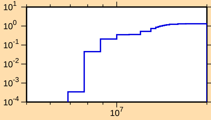
\sigma vs. E for ^{213}\text{Ra}(n,2n)
