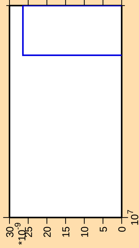
\Delta\sigma/\sigma vs. E for ^{213}\text{Ra}(\text{mt } 42)
