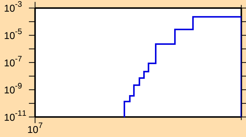
\sigma vs. E for ^{213}\text{Ra}(n,2np)
