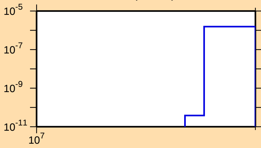
\sigma vs. E for ^{213}\text{Ra}(n,3n\alpha)
