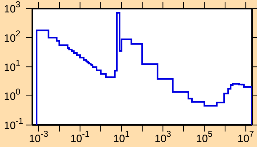
\sigma vs. E for ^{213}\text{Ra}(n,\text{nonel.})
