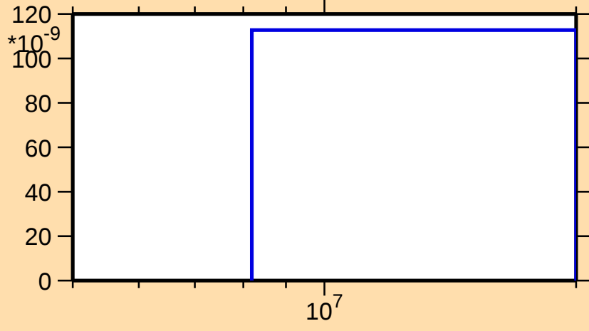
\sigma vs. E for ^{213}\text{Ra}(n,\text{nd})
