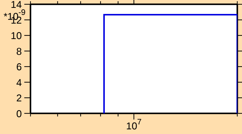
\sigma vs. E for ^{213}\text{Ra}(n,3n\alpha)
