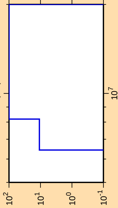
\Delta\sigma/\sigma vs. E for ^{213}\text{Ra}(n,t)
