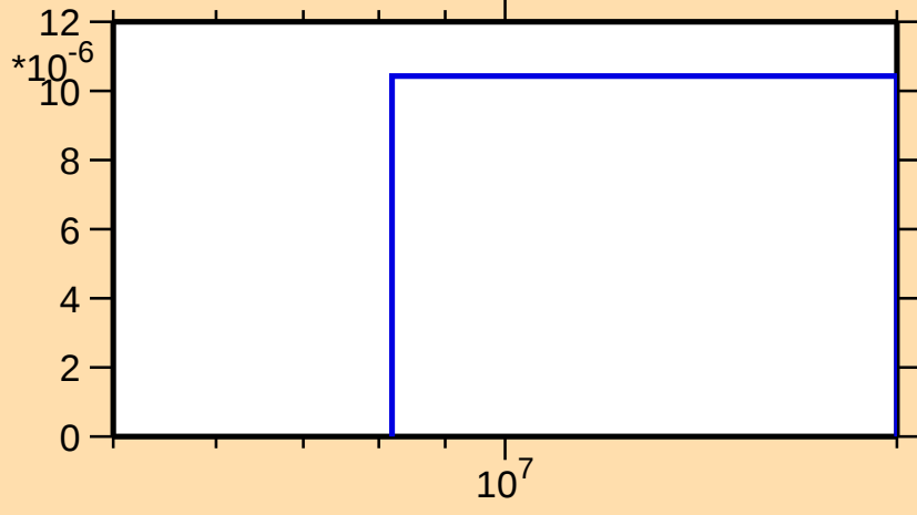
\sigma vs. E for ^{213}\text{Ra}(n,2n\alpha)
