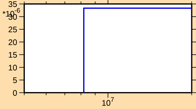
\sigma vs. E for ^{213}\text{Ra}(n,3n)
