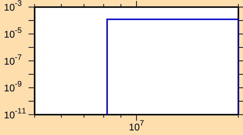
\sigma vs. E for ^{213}\text{Ra}(n,t)
