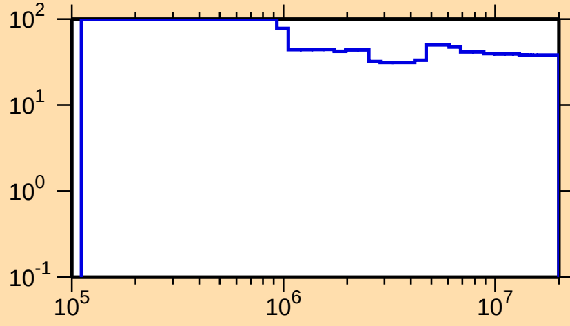
\Delta\sigma/\sigma vs. E for ^{222}\text{Ra}(n,n_1)
