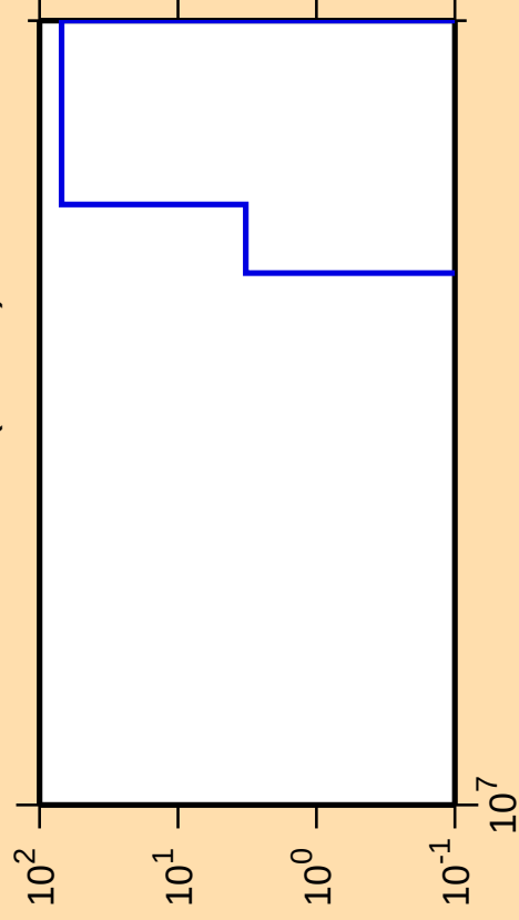
\Delta\sigma/\sigma vs. E for ^{222}\text{Ra}(\text{mt } 45)
