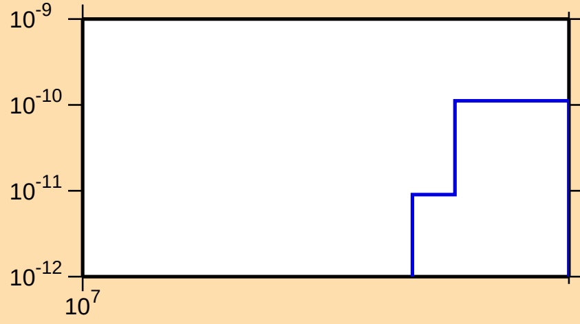
\sigma vs. E for ^{222}\text{Ra}(\text{mt117})
