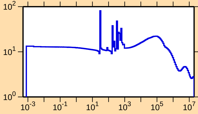
\sigma vs. E for ^{222}\text{Ra}(n,\text{el.})
