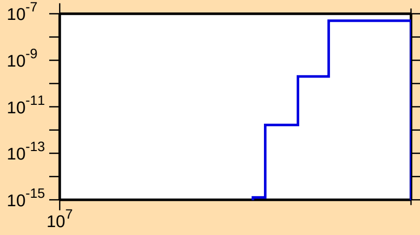
\sigma vs. E for ^{222}\text{Ra}(n,2np)
