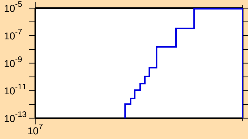
\sigma vs. E for ^{222}\text{Ra}(n,\text{nt})
