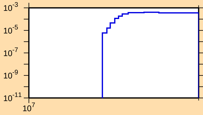
\sigma vs. E for ^{222}\text{Ra}(n,3n\alpha)
