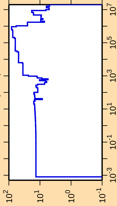
\Delta\sigma/\sigma vs. E for ^{222}\text{Ra}(n,\text{el.})
