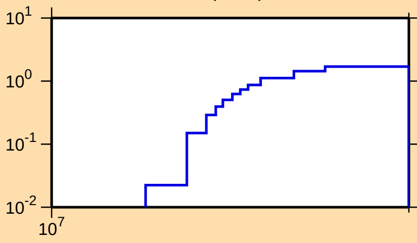
\sigma vs. E for ^{222}\text{Ra}(n,3n)
