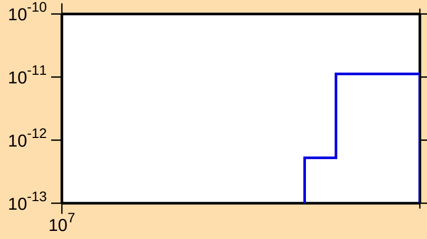
\sigma vs. E for ^{222}\text{Ra}(\text{mt } 45)
