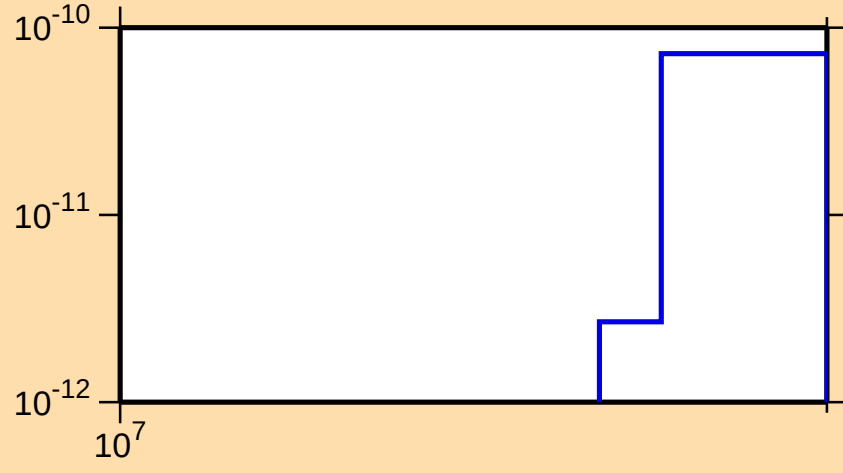
\sigma vs. E for ^{222}\text{Ra}(n,\text{He}3)
