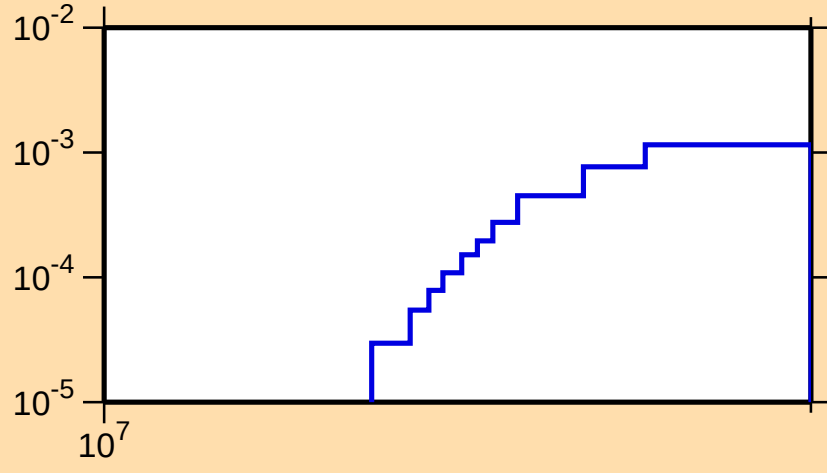
\sigma vs. E for ^{222}\text{Ra}(n,p\alpha)
