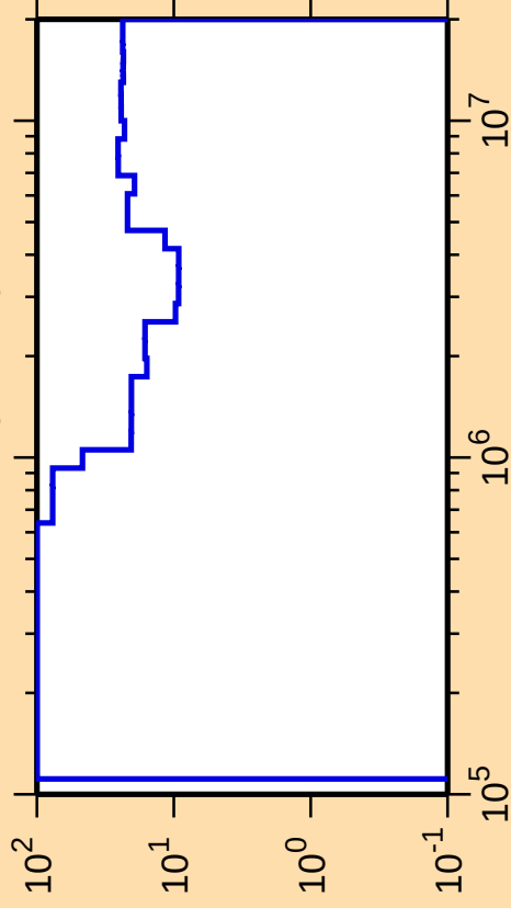
\Delta\sigma/\sigma vs. E for ^{222}\text{Ra}(n,\text{inel.})
