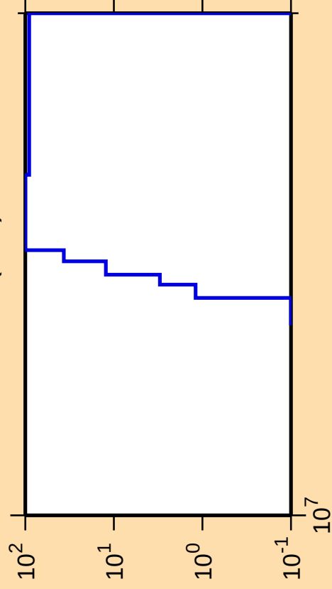
\Delta\sigma/\sigma vs. E for ^{222}\text{Ra}(n,\text{nt})
