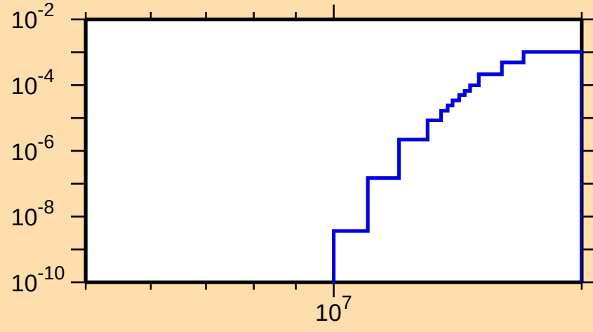
\sigma vs. E for ^{222}\text{Ra}(n,t)
