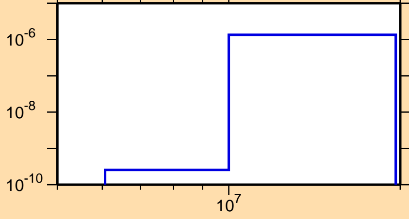
\sigma vs. E for ^{222}\text{Ra}(n,2n\alpha)
