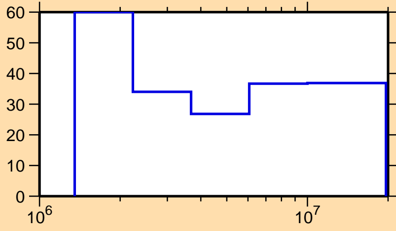
\Delta\sigma/\sigma vs. E for ^{222}\text{Ra}(n,n\text{cont.})
