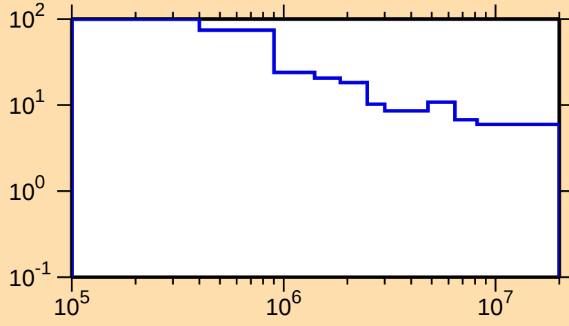
\Delta\sigma/\sigma vs. E for ^{222}\text{Ra}(n,\text{nonel.})
