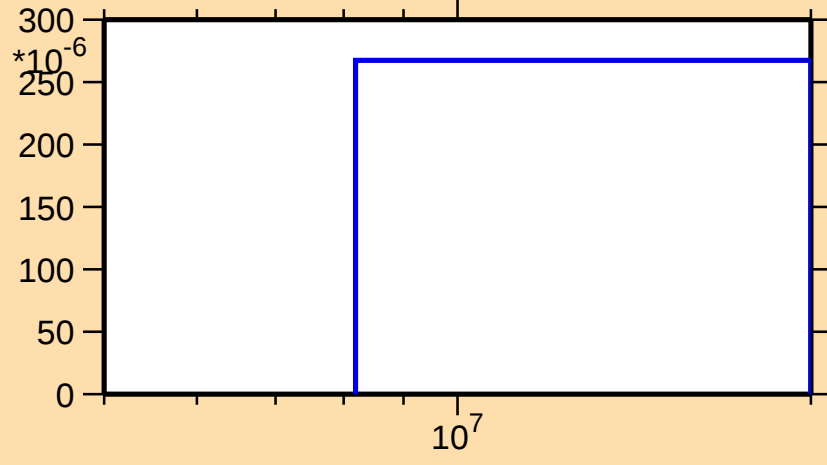
\sigma vs. E for ^{222}\text{Ra}(n,np)
