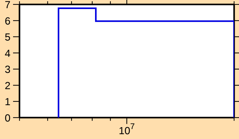
\Delta\sigma/\sigma vs. E for ^{222}\text{Ra}(n,\text{nonel.})
