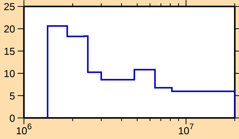
\Delta\sigma/\sigma vs. E for ^{222}\text{Ra}(n,n\text{nonel.})
