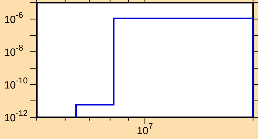
\sigma vs. E for ^{222}\text{Ra}(n,2n\alpha)
