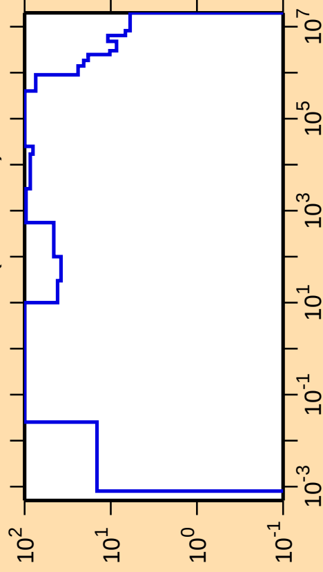
\Delta\sigma/\sigma vs. E for ^{222}\text{Ra}(n,\text{nonel.})
