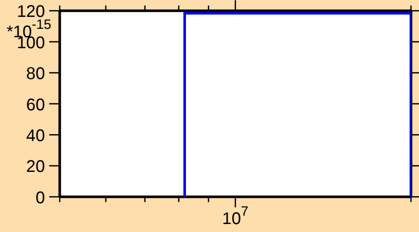
\sigma vs. E for ^{222}\text{Ra}(\text{mt } 45)
