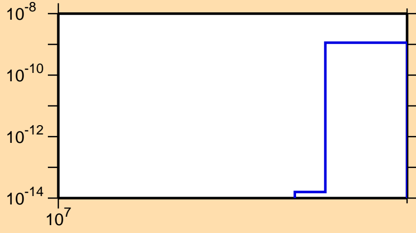
\sigma vs. E for ^{228}\text{Ra}(n,2np)
