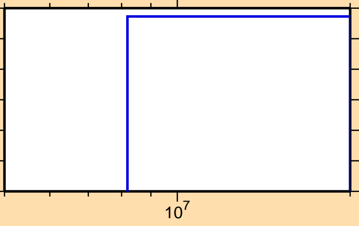
\sigma vs. E for ^{228}\text{Ra}(n,t)
