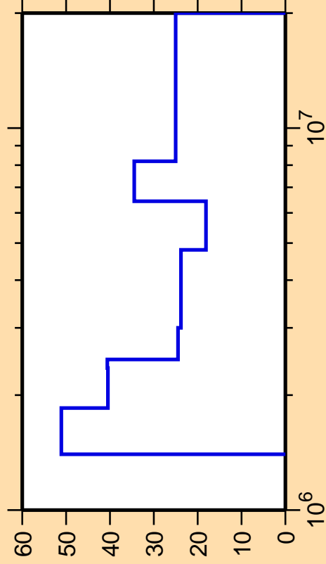
\Delta\sigma/\sigma vs. E for ^{228}\text{Ra}(n,\text{ncont.})
