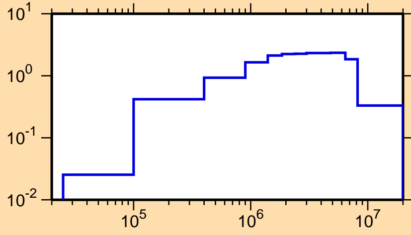
\sigma vs. E for ^{228}\text{Ra}(n,\text{inel.})
