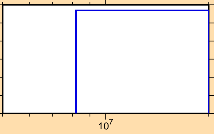
\sigma vs. E for ^{228}\text{Ra}(n,nt)
