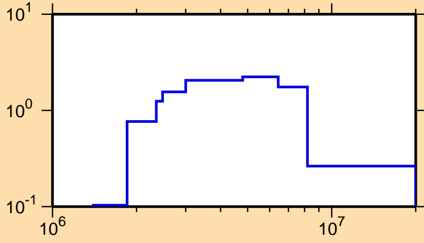
\sigma vs. E for ^{228}\text{Ra}(n,n\text{cont.})
