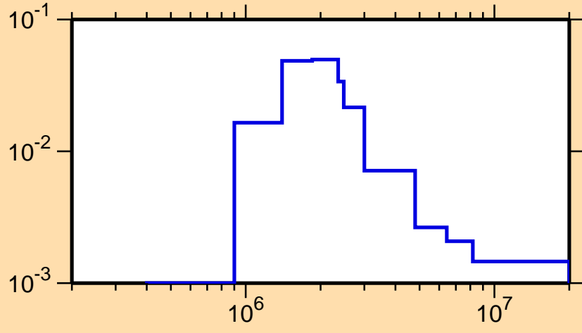
\sigma vs. E for ^{228}\text{Ra}(n,n_3)
