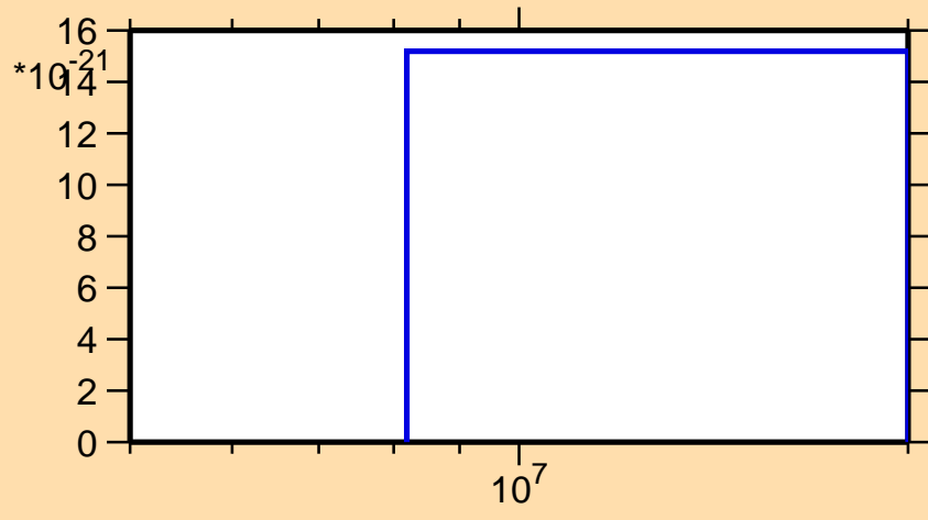
\sigma vs. E for ^{228}\text{Ra} (mt 42)
