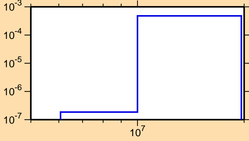
\sigma vs. E for ^{230}\text{Ra}(n,n\alpha)
