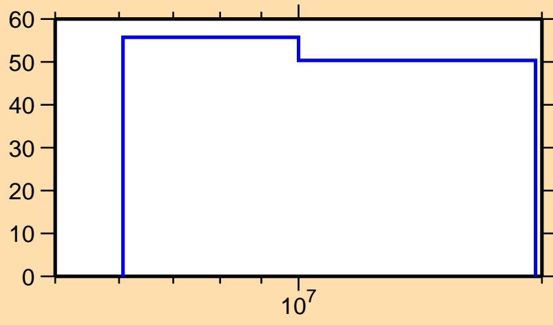
\Delta\sigma/\sigma vs. E for ^{230}\text{Ra}(n,2n)
