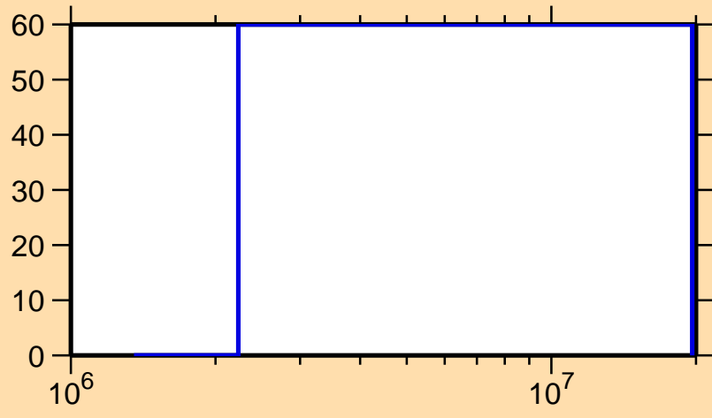
\Delta\sigma/\sigma vs. E for ^{230}\text{Ra}(n, f)
