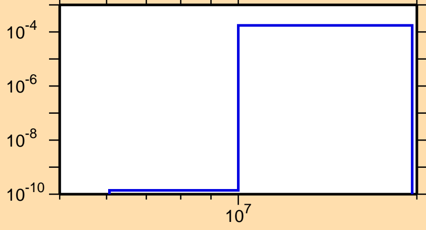
\sigma vs. E for ^{230}\text{Ra}(n,p)
