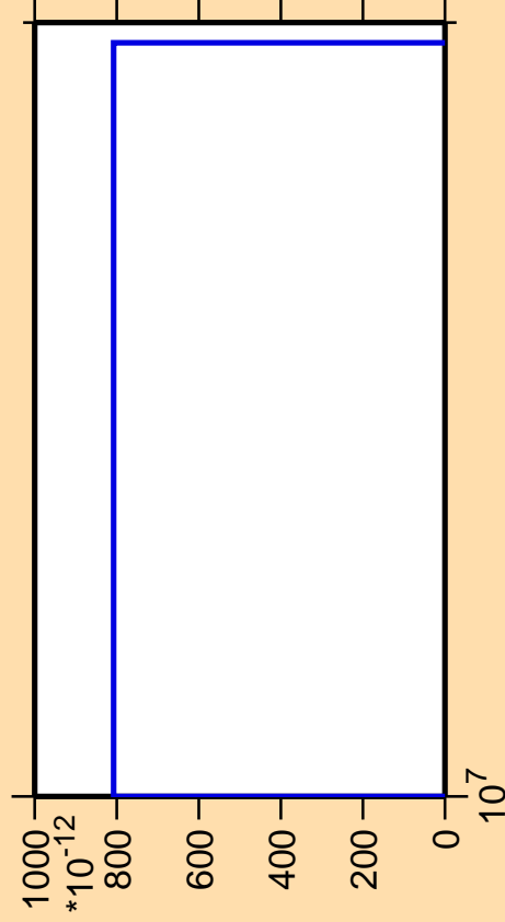
\Delta\sigma/\sigma vs. E for ^{230}\text{Ra} (mt 42)
