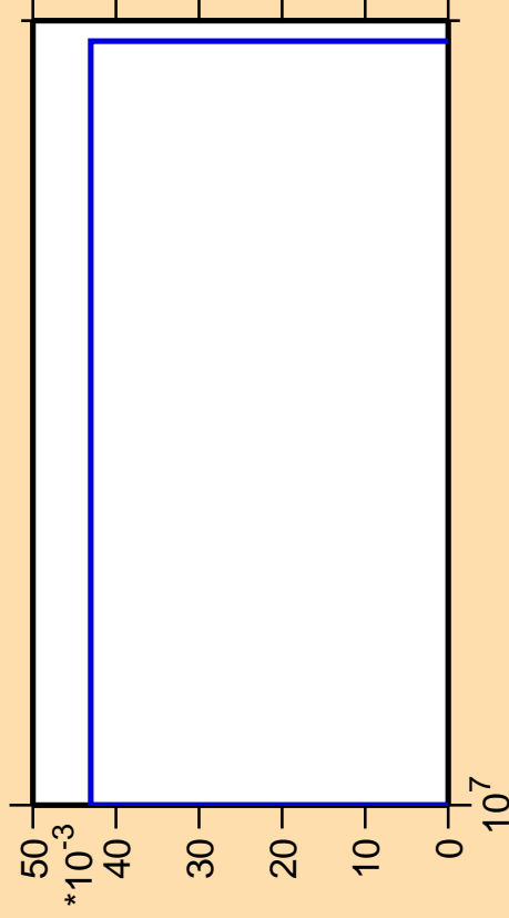
\Delta\sigma/\sigma vs. E for ^{230}\text{Ra}(n,3n\alpha)
