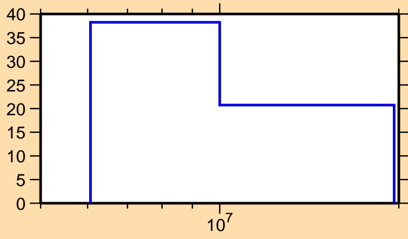
\Delta\sigma/\sigma vs. E for ^{230}\text{Ra}(n,\text{el.})
