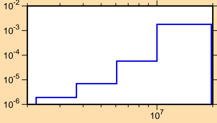
\sigma vs. E for ^{230}\text{Ra}(n,\alpha)
