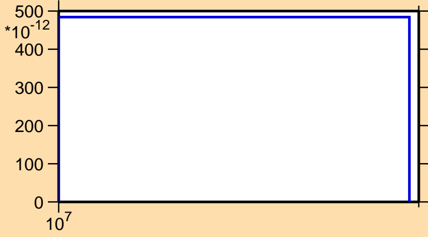
\sigma vs. E for ^{230}\text{Ra}(n,\text{nd})
