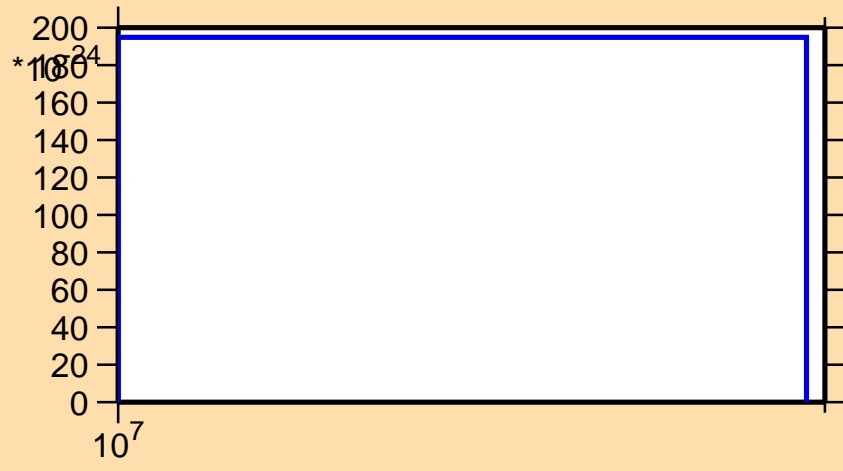
\sigma vs. E for ^{230}\text{Ra} (mt 42)
