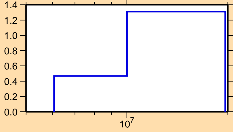
\sigma vs. E for ^{230}\text{Ra}(n,2n)
