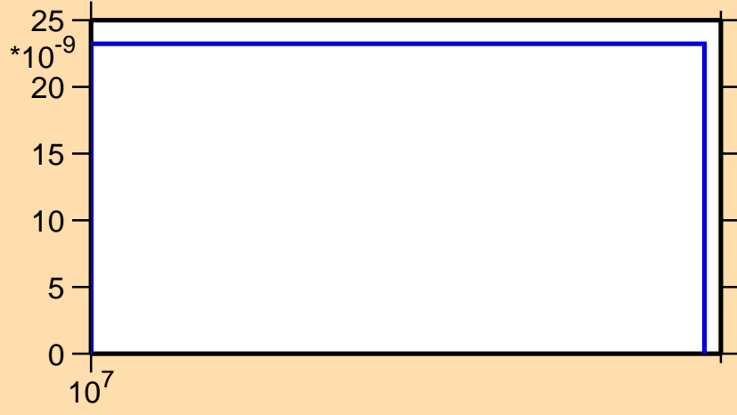
\sigma vs. E for ^{230}\text{Ra}(n,nt)
