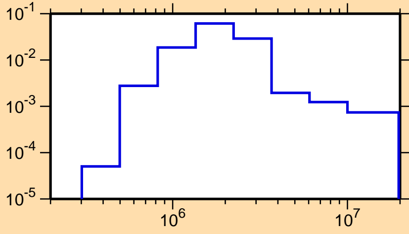
\sigma vs. E for ^{230}\text{Ra}(n,n_3)
