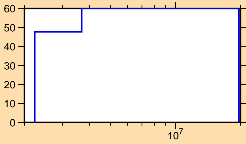
\Delta\sigma/\sigma vs. E for ^{230}\text{Ra}(n,n_1)
