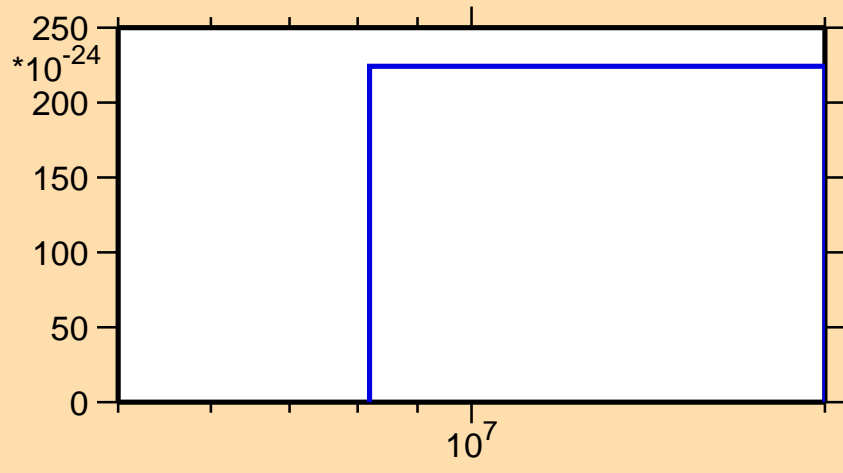
\sigma vs. E for ^{230}\text{Ra} (mt 42)
