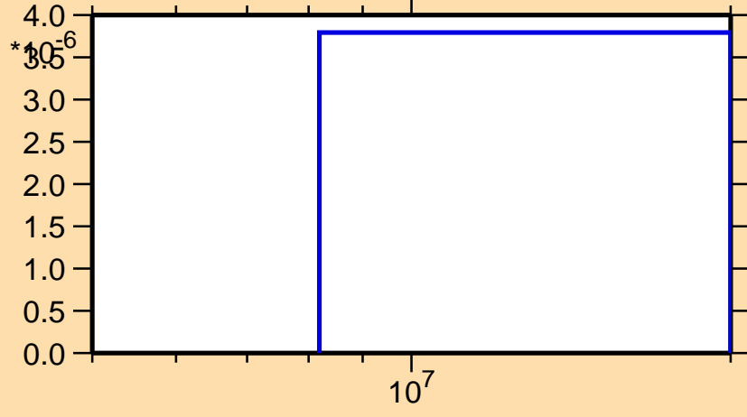
\sigma vs. E for ^{230}\text{Ra}(n,np)
