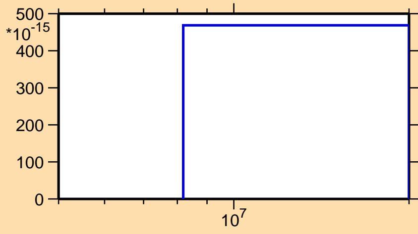
\sigma vs. E for ^{230}\text{Ra}(n,2n\alpha)
