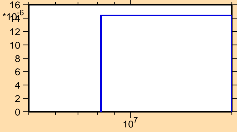
\sigma vs. E for ^{230}\text{Ra}(n,d)
