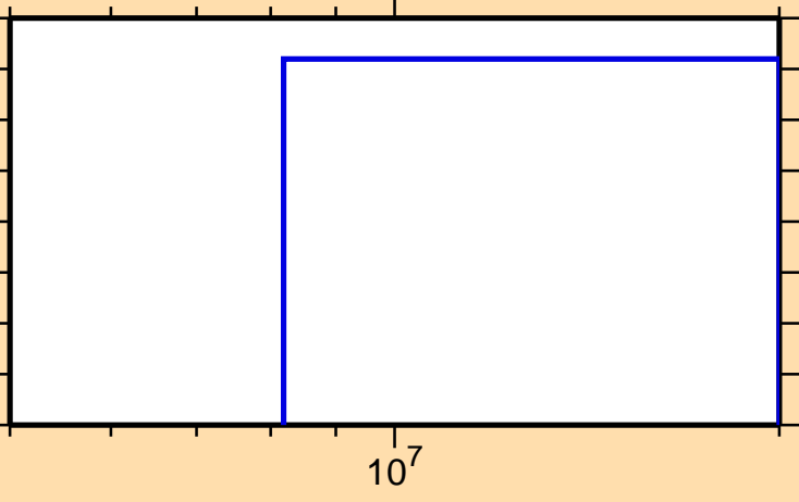
\sigma vs. E for ^{230}\text{Ra}(n,d)
