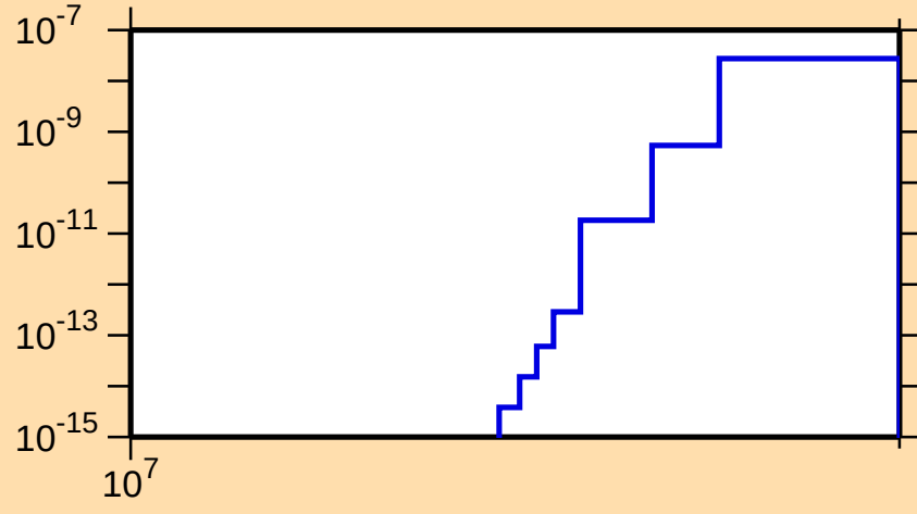
\sigma vs. E for ^{104}\text{Rh}(n,\text{He3})
