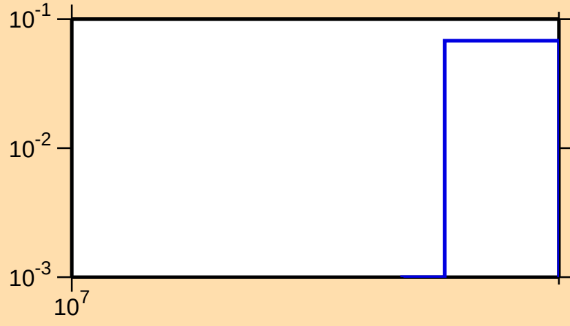
\sigma vs. E for ^{104}\text{Rh}(n,3n)
