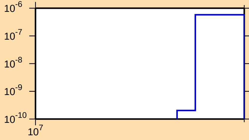
\sigma vs. E for ^{104}\text{Rh}(n,\text{nt})
