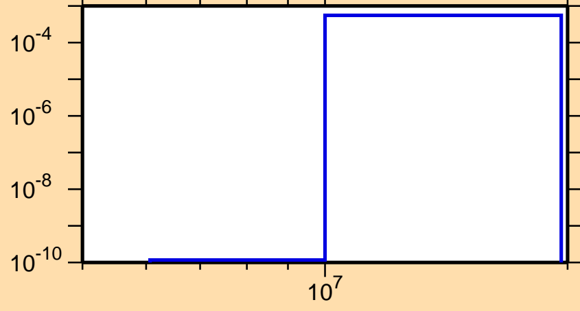
\sigma vs. E for ^{110}\text{Rh}(n,d)
