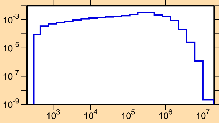
\sigma vs. E for ^{110}\text{Rh}(n,n_4)
