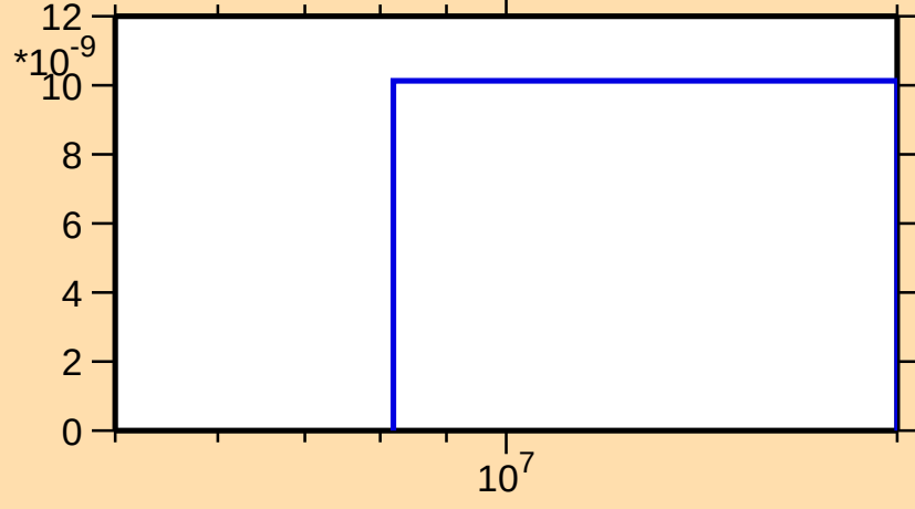
\sigma vs. E for ^{110}\text{Rh}(n,2np)
