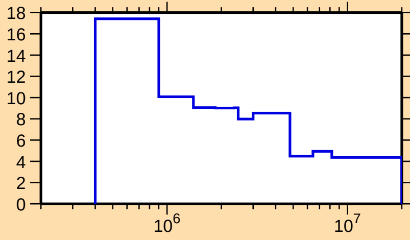
\Delta\sigma/\sigma vs. E for ^{110}\text{Rh}(n,n\text{nonel.})
