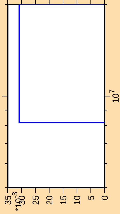
\Delta\sigma/\sigma vs. E for ^{110}\text{Rh}(n,\text{He3})
