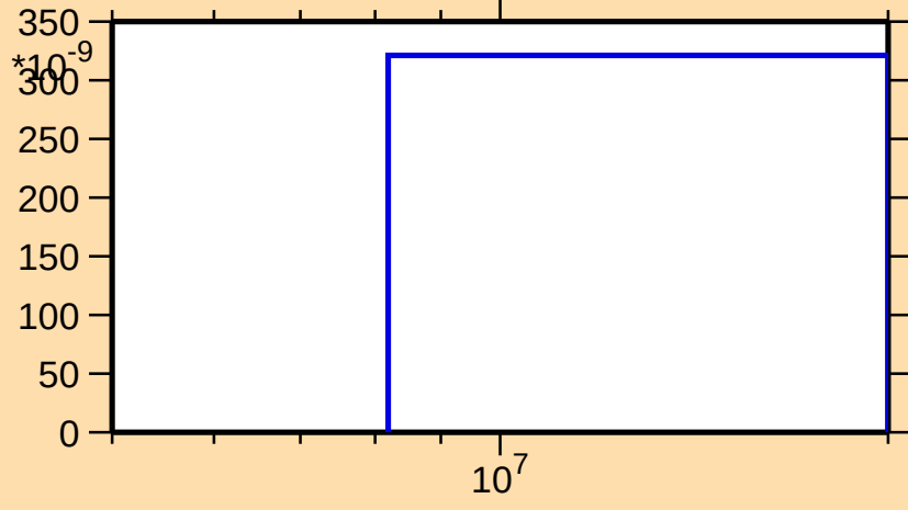
\sigma vs. E for ^{110}\text{Rh}(n,\text{nd})
