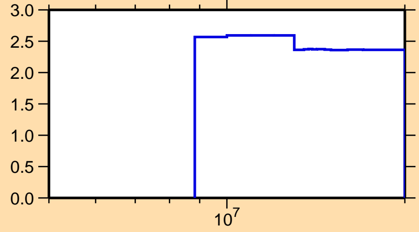
\Delta\sigma/\sigma vs. E for ^{95}\text{Ru}(n,\text{nonel.})
