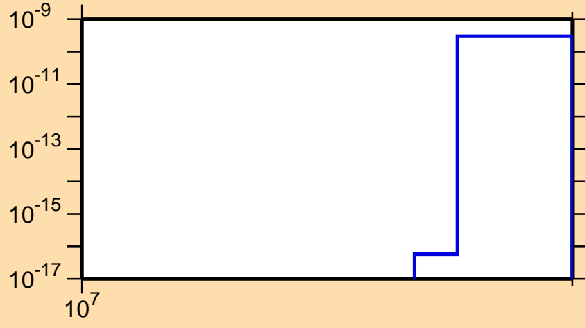
\sigma vs. E for ^{96}\text{Ru}(n,\text{pt})
