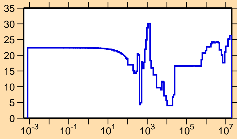
\Delta\sigma/\sigma vs. E for ^{96}\text{Ru}(n,\gamma)
