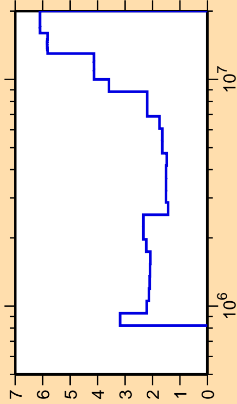
\Delta\sigma/\sigma vs. E for ^{96}\text{Ru}(n,\text{inel.})
