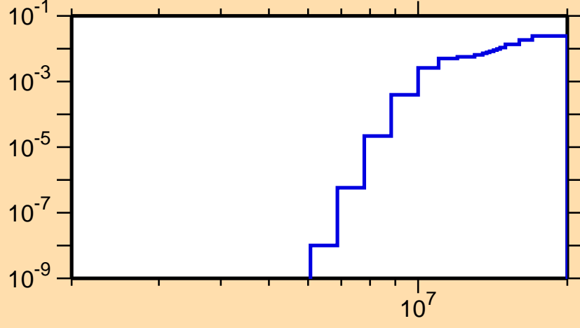
\sigma vs. E for ^{96}\text{Ru}(n,n\alpha)
