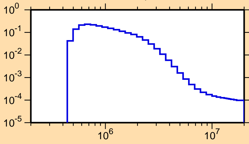
\sigma vs. E for ^{99}\text{Ru}(n,n_4)
