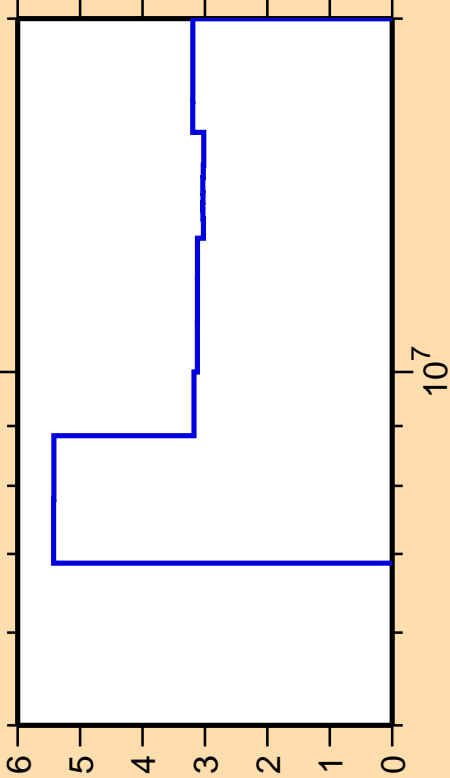
\Delta\sigma/\sigma vs. E for ^{99}\text{Ru}(n,2n)
