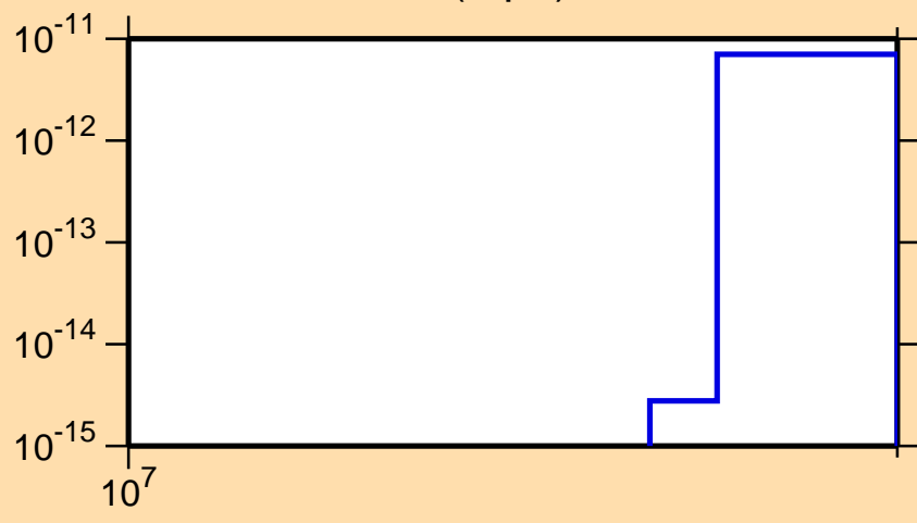
\sigma vs. E for ^{99}\text{Ru}(n,\text{pd})
