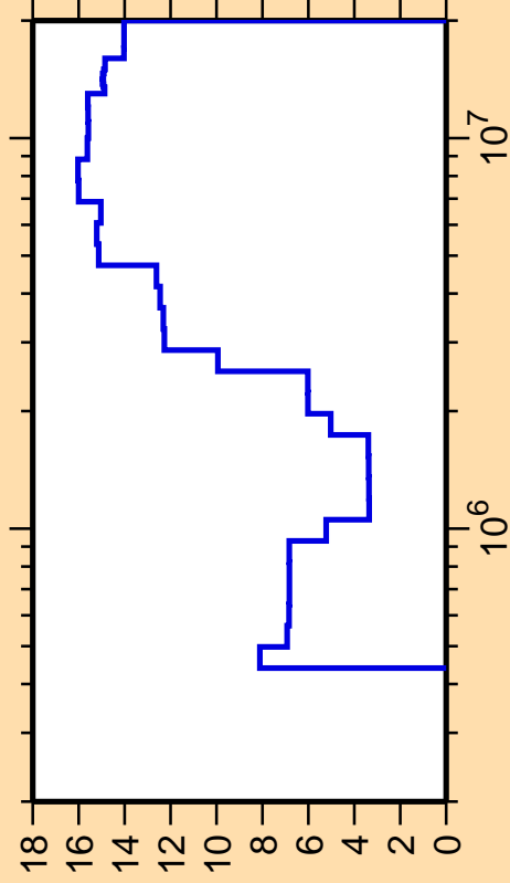
\Delta\sigma/\sigma vs. E for ^{99}\text{Ru}(n,n_4)
