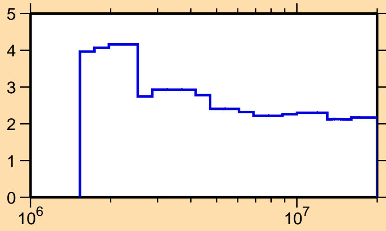
\Delta\sigma/\sigma vs. E for ^{99}\text{Ru}(n,n\text{nonel.})
