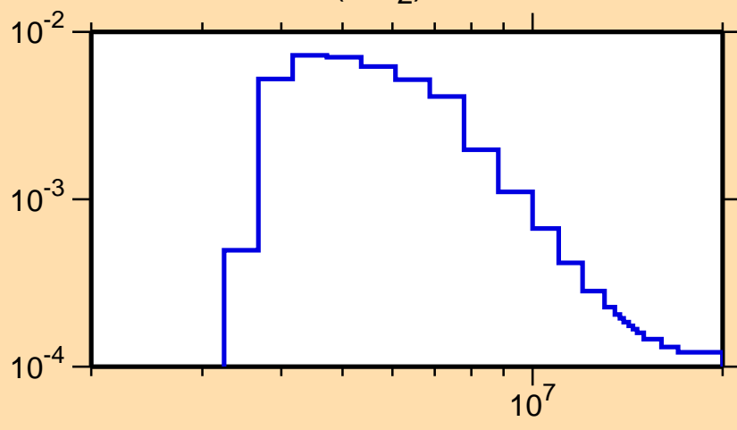
\sigma vs. E for ^{30}\text{S}(n,n_2)
