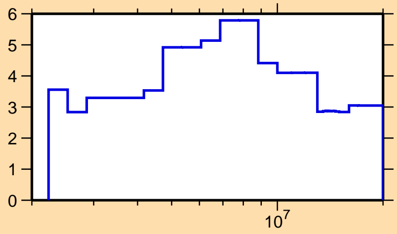
\Delta\sigma/\sigma vs. E for ^{30}\text{S}(n,\text{el.})
