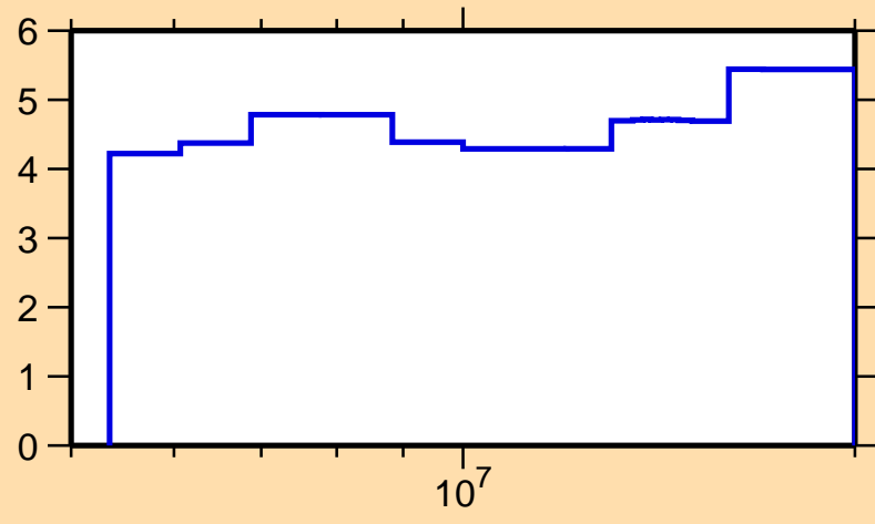
\Delta\sigma/\sigma vs. E for ^{30}\text{S}(n,n\text{onel.})
