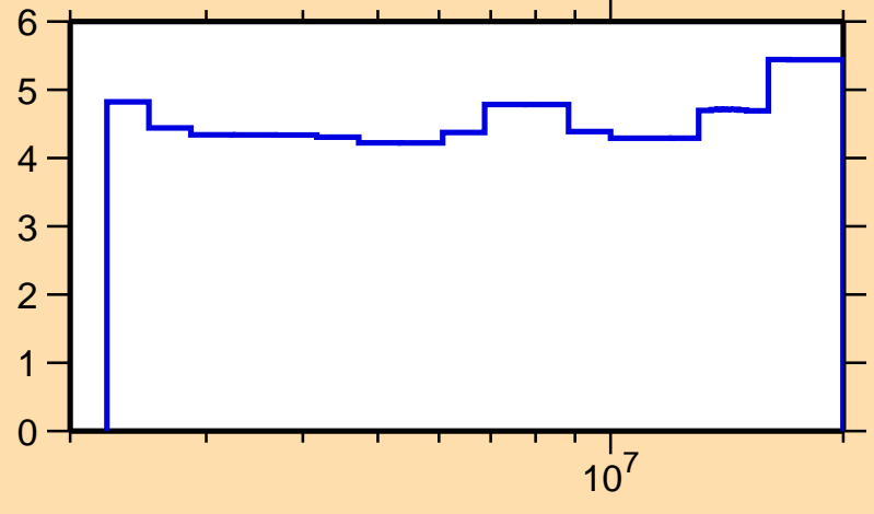
\Delta\sigma/\sigma vs. E for ^{30}\text{S}(n,\text{nonel.})
