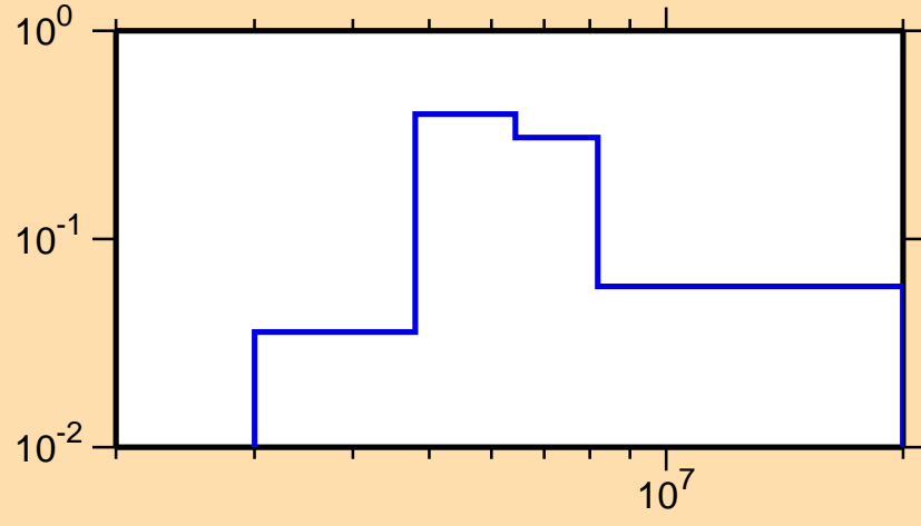
\sigma vs. E for ^{39}\text{S}(n,n\text{cont.})
