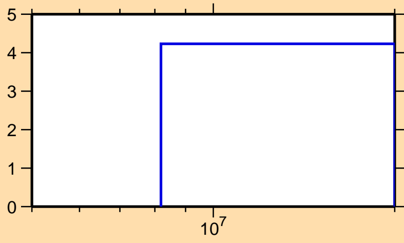
\Delta\sigma/\sigma vs. E for ^{39}\text{S}(n,el.)
