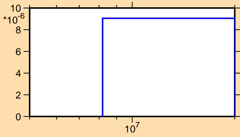
\sigma vs. E for ^{39}\text{S}(n,n\alpha)
