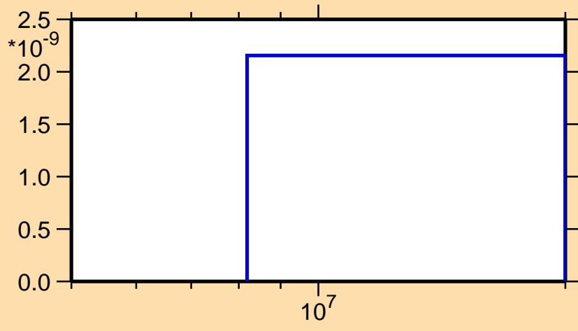
\sigma vs. E for ^{39}\text{S}(n,nd)
