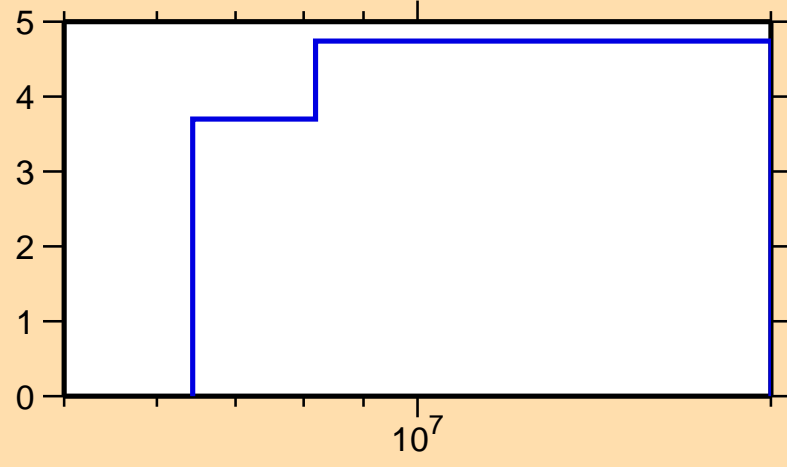
\Delta\sigma/\sigma vs. E for ^{39}\text{S}(n,2n)
