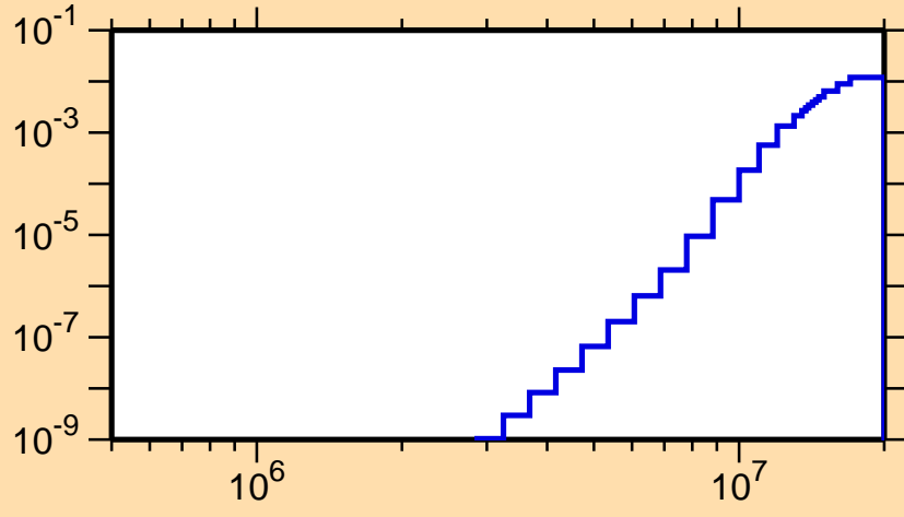
\sigma vs. E for ^{105}\text{Sb}(n,\text{He}3)
