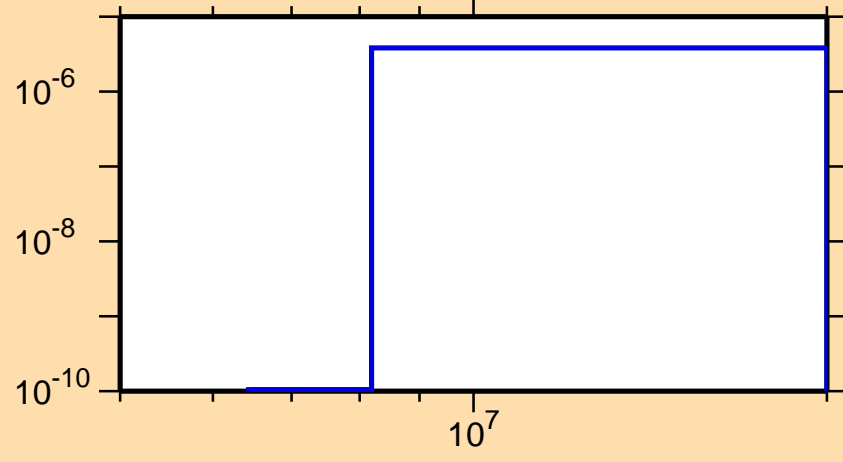
\sigma vs. E for ^{105}\text{Sb}(\text{mt117})
