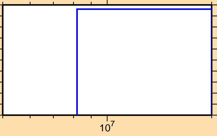
\sigma vs. E for ^{105}\text{Sb}(n,2np)
