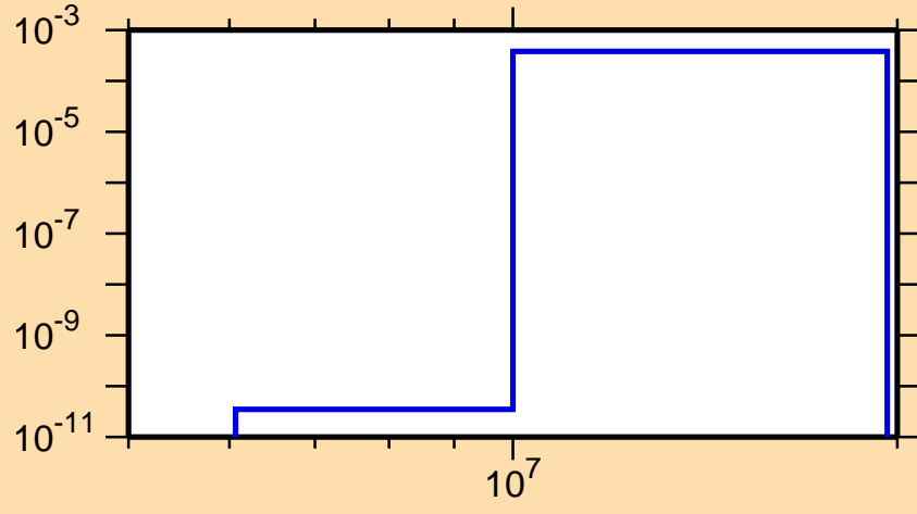
\sigma vs. E for ^{108}\text{Sb}(n,\text{pd})
