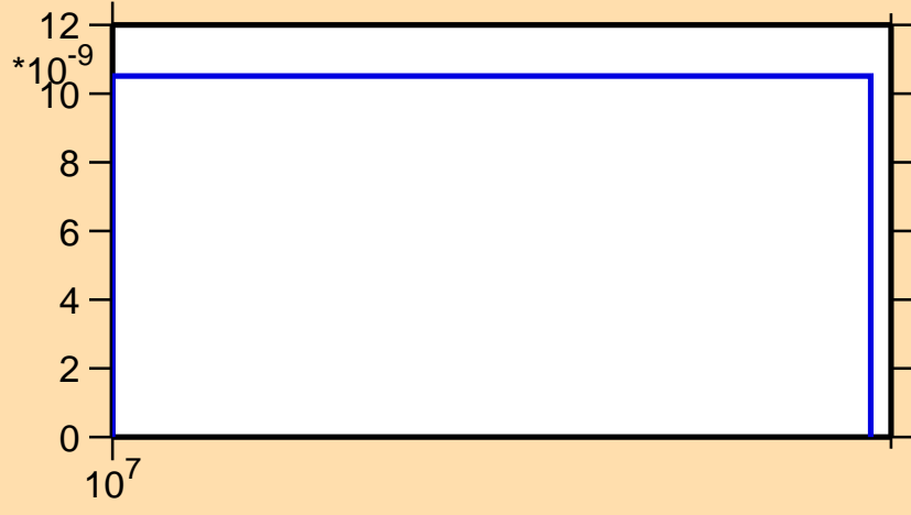
\sigma vs. E for ^{108}\text{Sb} (mt 34)
