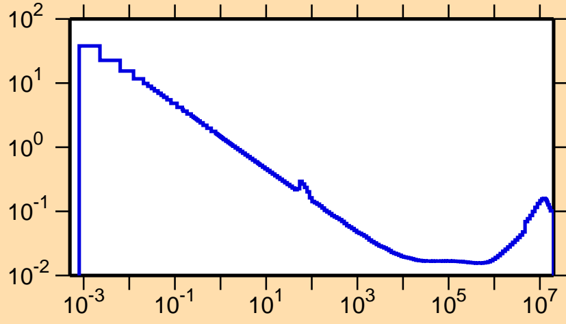
\sigma vs. E for ^{110}\text{Sb}(n,\alpha)
