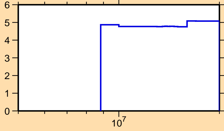
\Delta\sigma/\sigma vs. E for ^{110}\text{Sb}(n,\text{nonel.})
