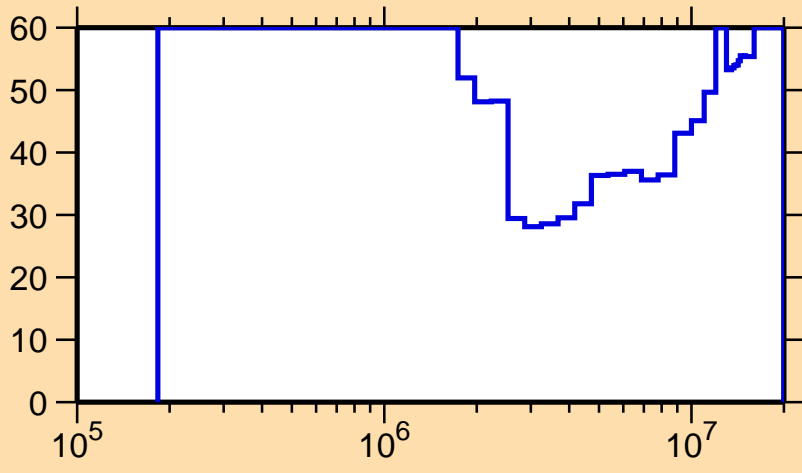
\Delta\sigma/\sigma vs. E for ^{110}\text{Sb}(n,n_1)
