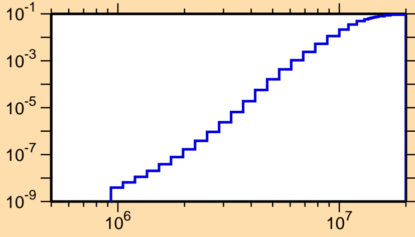
\sigma vs. E for ^{110}\text{Sb}(n,p\alpha)
