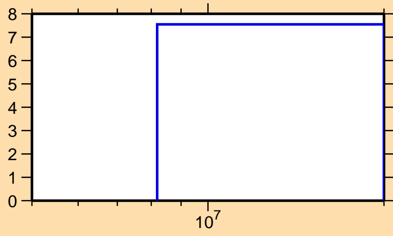
\Delta\sigma/\sigma vs. E for ^{110}\text{Sb}(n,\text{el.})
