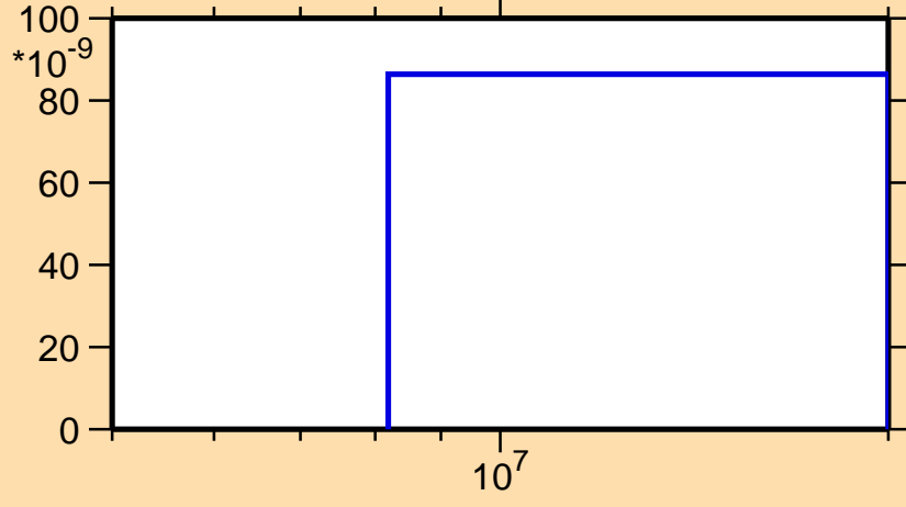
\sigma vs. E for ^{110}\text{Sb}(n,2n\alpha)
