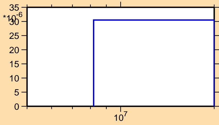
\sigma vs. E for ^{110}\text{Sb}(n,nd)
