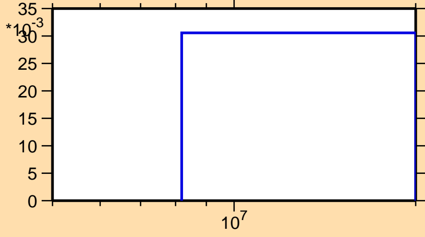
\sigma vs. E for ^{110}\text{Sb}(n,2n)
