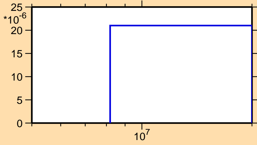
\sigma vs. E for ^{110}\text{Sb}(n,\text{pd})
