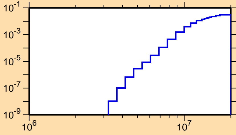
\sigma vs. E for ^{112}\text{Sb}(n,d)
