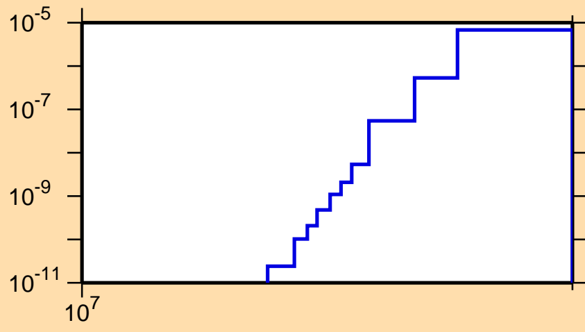
\sigma vs. E for ^{112}\text{Sb}(\text{mt } 45)
