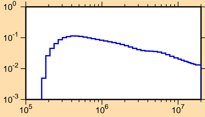
\sigma vs. E for ^{112}\text{Sb}(n,n_3)
