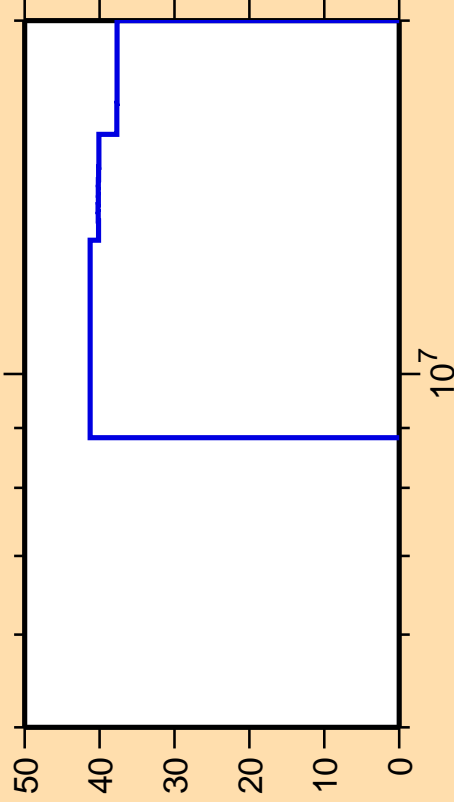
\Delta\sigma/\sigma vs. E for ^{112}\text{Sb}(n,2n)
