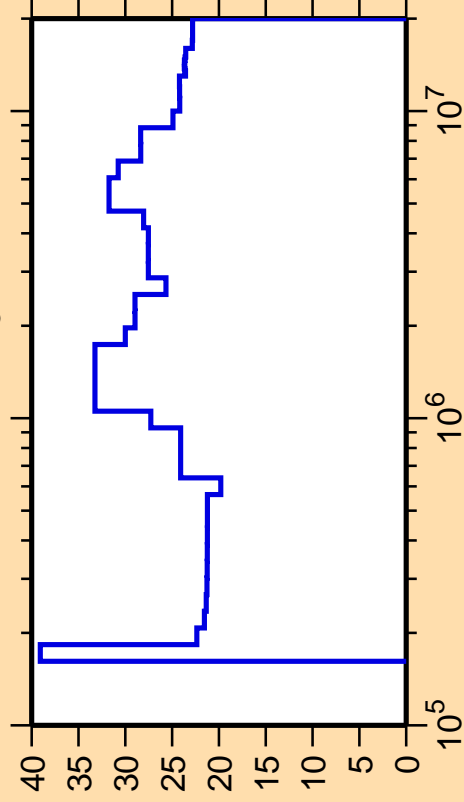
\Delta\sigma/\sigma vs. E for ^{112}\text{Sb}(n,n_3)
