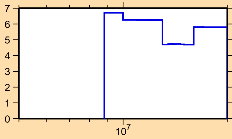
\Delta\sigma/\sigma vs. E for ^{112}\text{Sb}(n,\text{el.})
