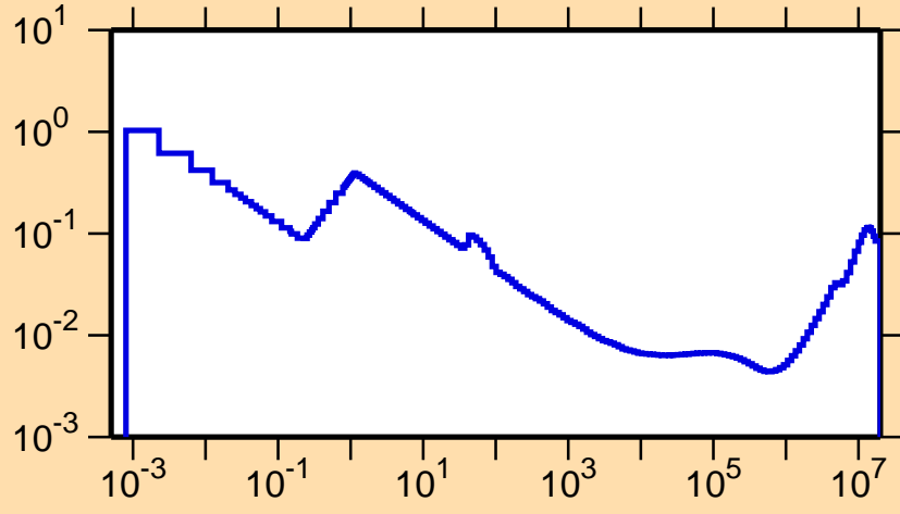
\sigma vs. E for ^{112}\text{Sb}(n,\alpha)
