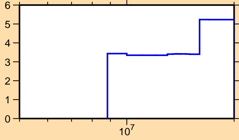
\Delta\sigma/\sigma vs. E for ^{112}\text{Sb}(n,\text{tot.})
