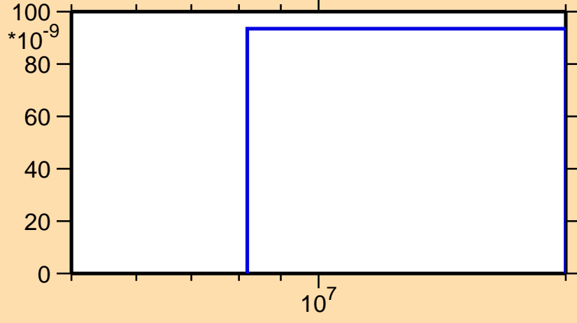
\sigma vs. E for ^{112}\text{Sb}(n,pd)
