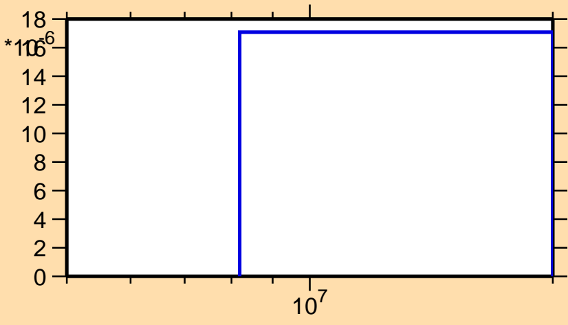
\sigma vs. E for ^{112}\text{Sb}(n,\text{nd})
