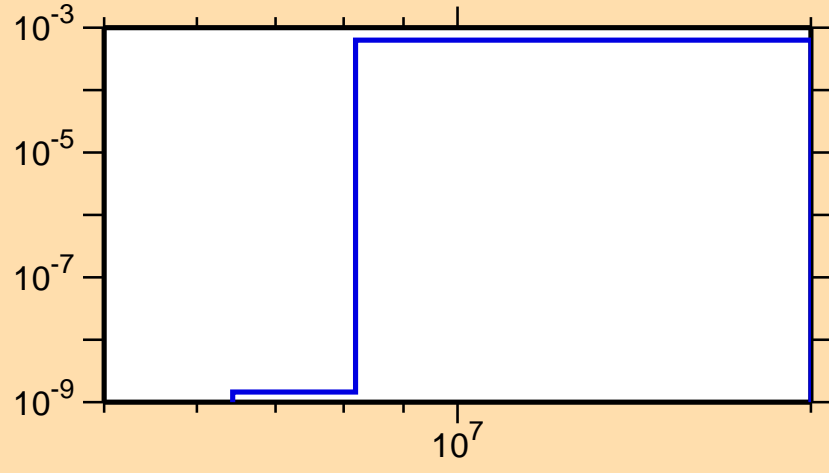
\sigma vs. E for ^{117}\text{Sb}(n,n\alpha)
