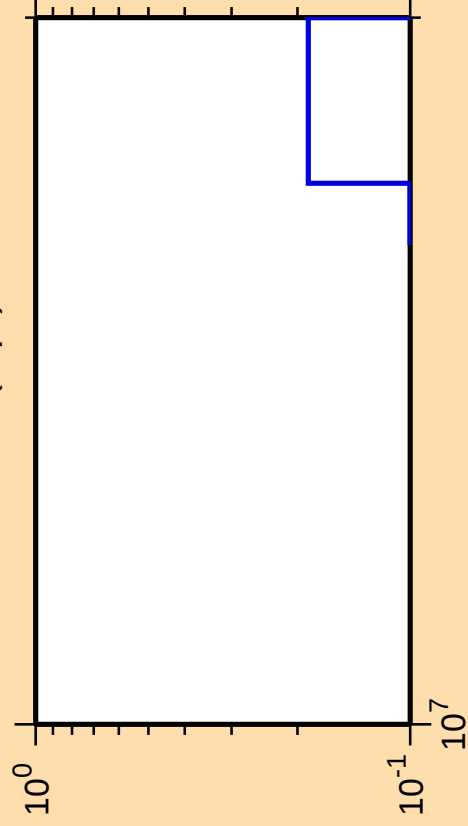
\Delta\sigma/\sigma vs. E for ^{118}\text{Sb}(n,\text{pt})
