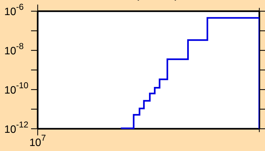
\sigma vs. E for ^{118}\text{Sb}(n,\text{He}3)
