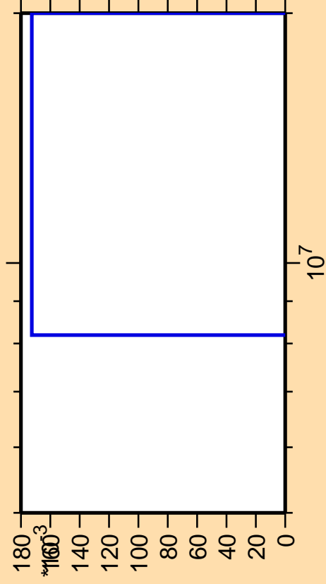
\Delta\sigma/\sigma vs. E for ^{121}\text{Sb}(n,p\alpha)
