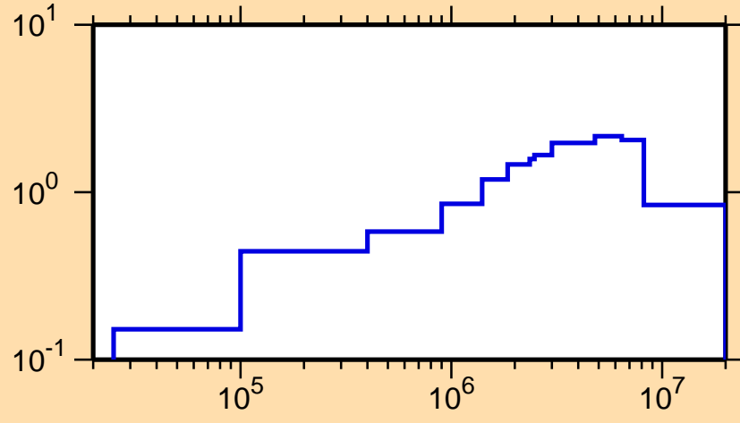
\sigma vs. E for ^{121}\text{Sb}(n,\text{inel.})
