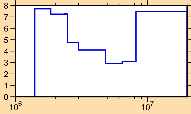
\Delta\sigma/\sigma vs. E for ^{121}\text{Sb}(n,\text{inel.})
