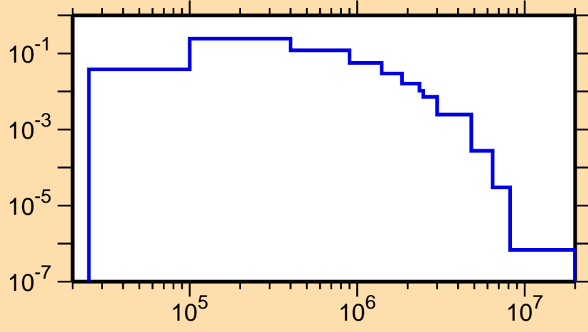
\sigma vs. E for ^{122}\text{Sb}(n,n_1)
