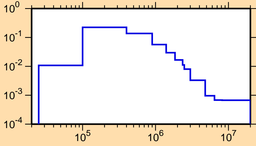
\sigma vs. E for ^{122}\text{Sb}(n,n_2)
