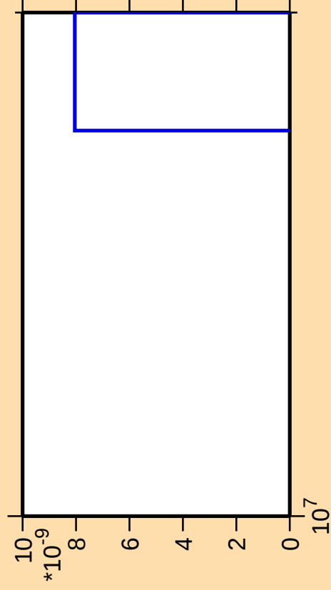
\Delta\sigma/\sigma vs. E for ^{122}\text{Sb} (mt 11)
