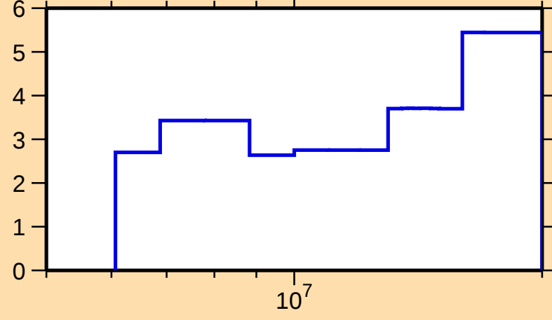
\Delta\sigma/\sigma vs. E for ^{122}\text{Sb}(n,\text{el.})
