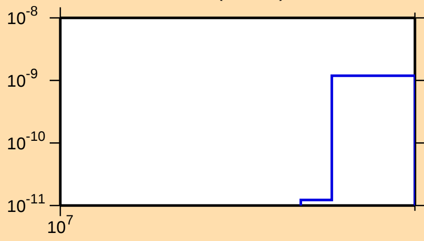
\sigma vs. E for ^{122}\text{Sb}(n,\text{He3})
