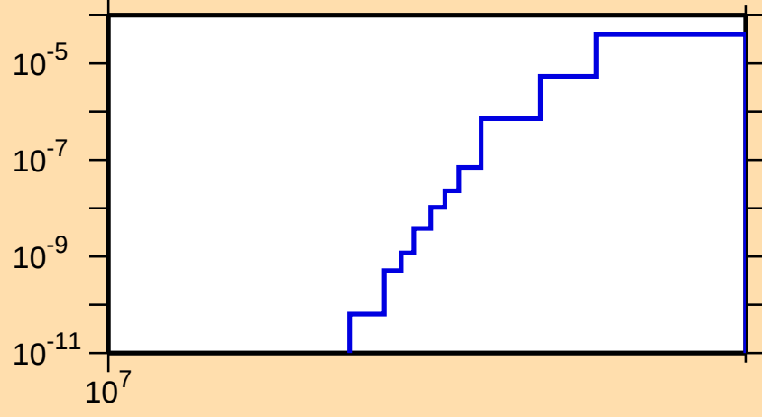
\sigma vs. E for ^{122}\text{Sb}(n,\text{nd})
