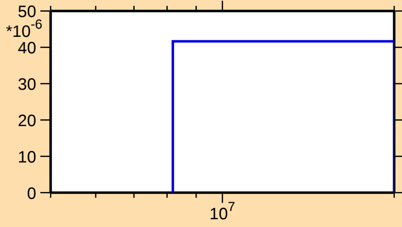
\sigma vs. E for ^{122}\text{Sb}(n,n\alpha)
