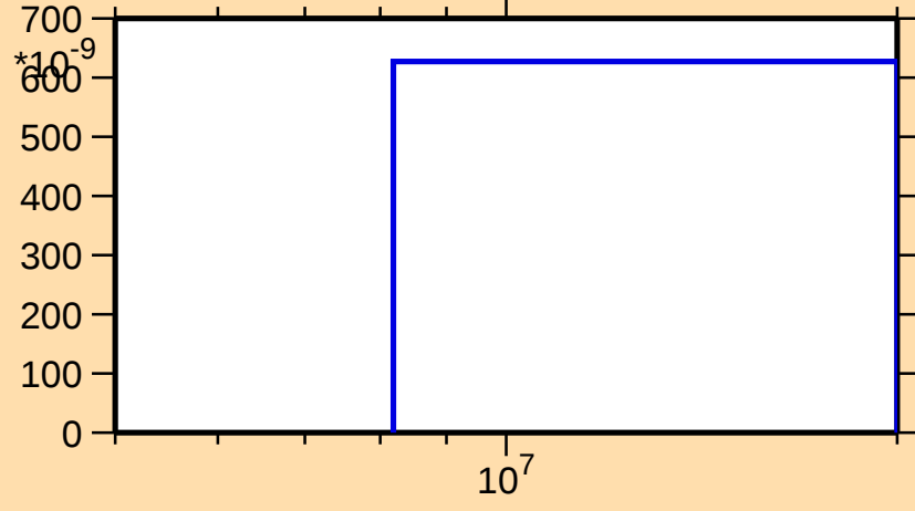
\sigma vs. E for ^{122}\text{Sb}(n,nd)
