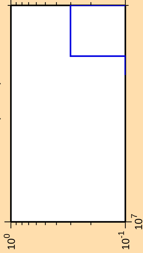
\Delta\sigma/\sigma vs. E for ^{125}\text{Sb}(n,2n\alpha)
