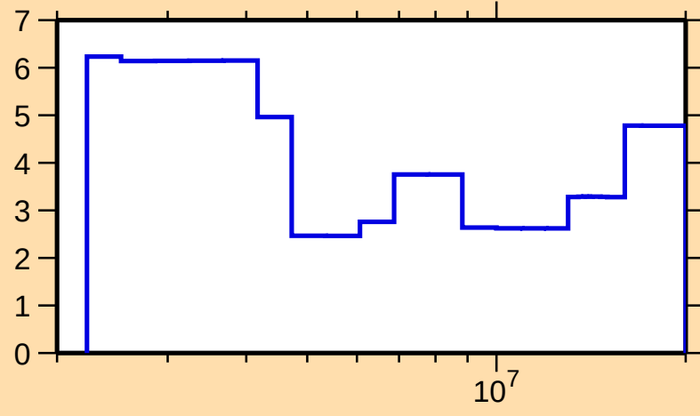
\Delta\sigma/\sigma vs. E for ^{125}\text{Sb}(n,\text{el.})
