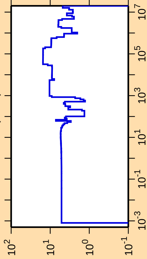
\Delta\sigma/\sigma vs. E for ^{125}\text{Sb}(n,\text{el.})
