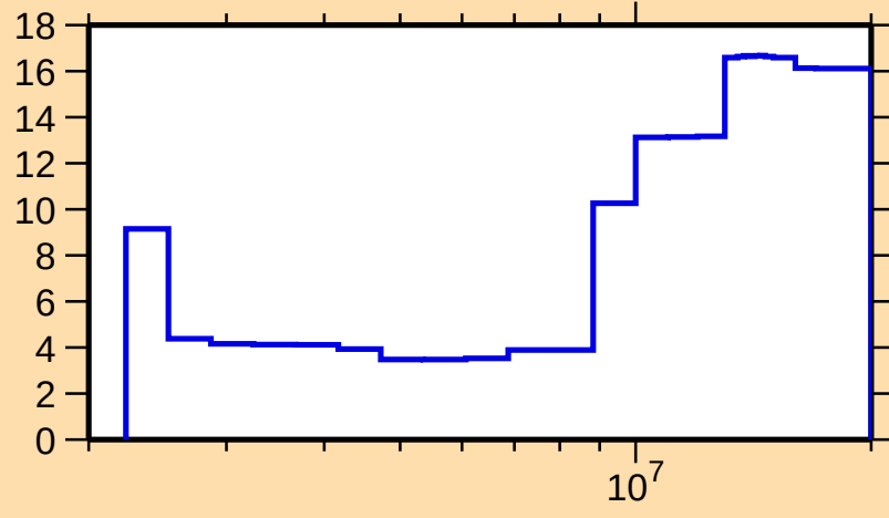
\Delta\sigma/\sigma vs. E for ^{125}\text{Sb}(n,n\text{cont.})
