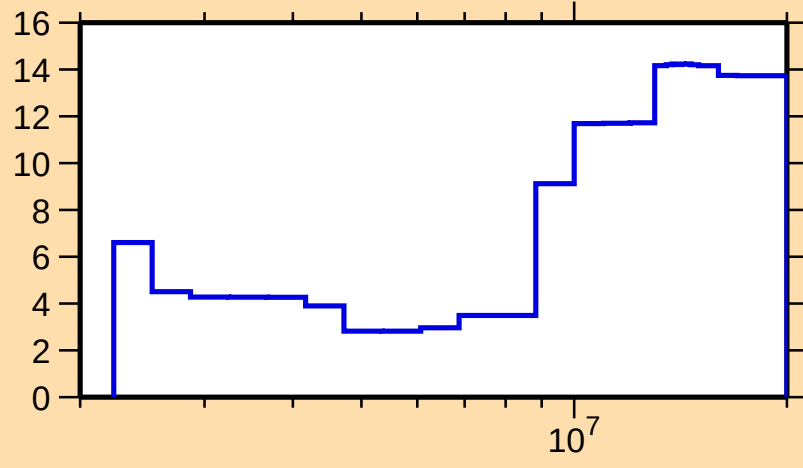
\Delta\sigma/\sigma vs. E for ^{125}\text{Sb}(n,\text{inel.})
