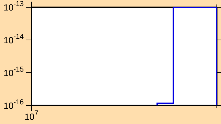
\sigma vs. E for ^{125}\text{Sb}(n,2n\alpha)
