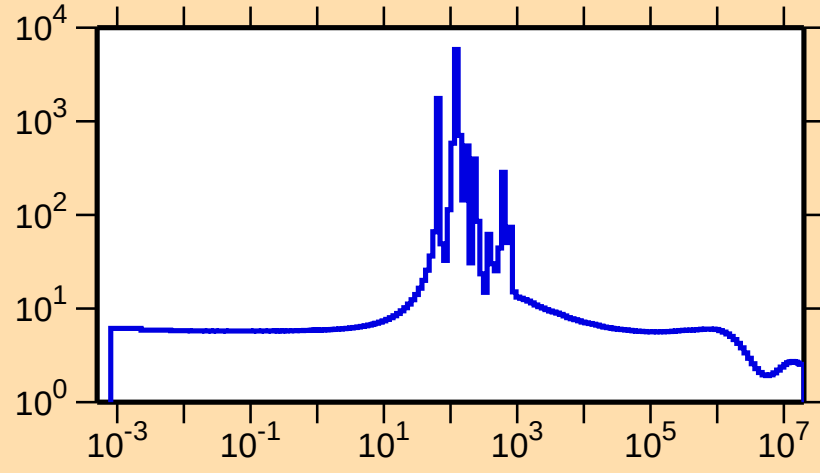
\sigma vs. E for ^{125}\text{Sb}(n,\text{el.})
