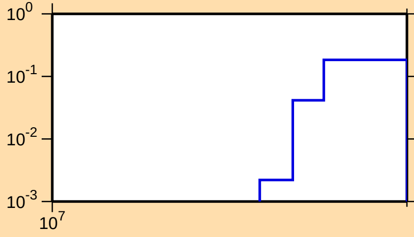
\sigma vs. E for ^{125}\text{Sb}(n,3n)
