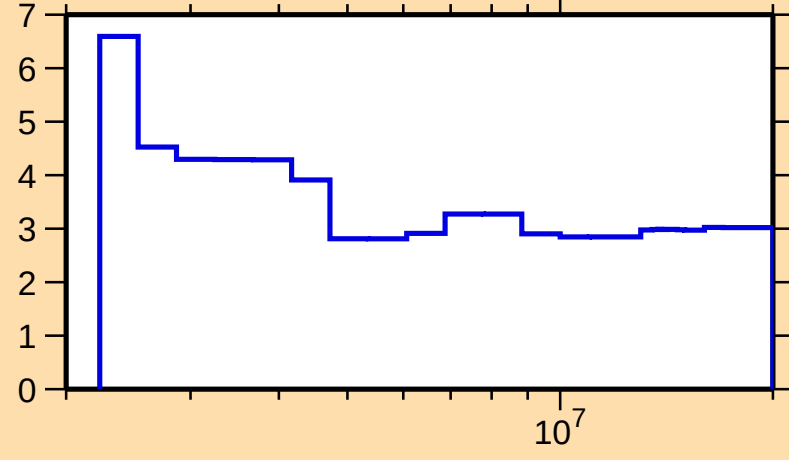
\Delta\sigma/\sigma vs. E for ^{125}\text{Sb}(n,n\text{onel.})
