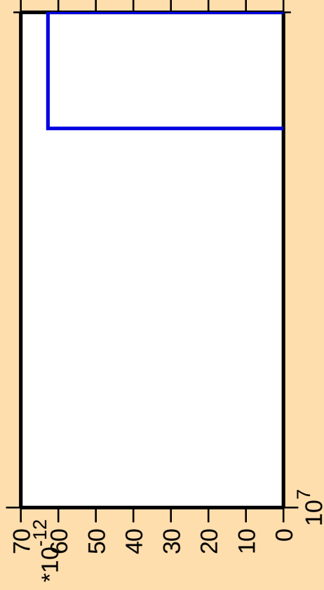
\Delta\sigma/\sigma vs. E for ^{125}\text{Sb}(\text{mt 11})
