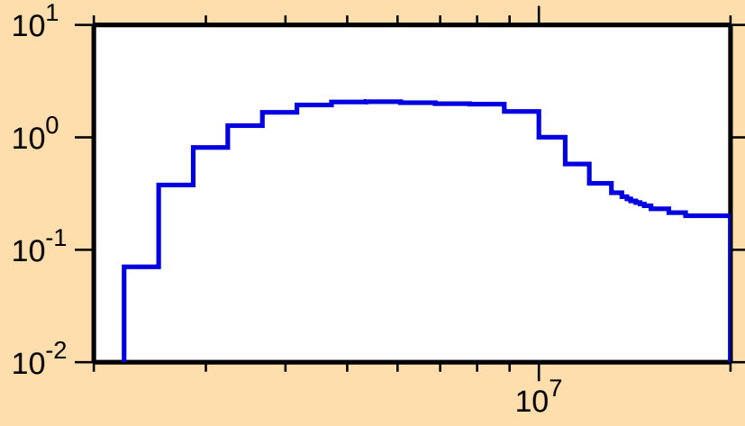
\sigma vs. E for ^{125}\text{Sb}(n,n\text{cont.})
