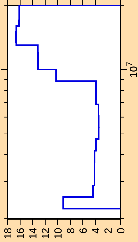
\Delta\sigma/\sigma vs. E for ^{125}\text{Sb}(n,n\text{cont.})
