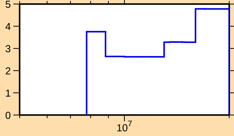
\Delta\sigma/\sigma vs. E for ^{125}\text{Sb}(n,\text{el.})
