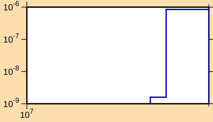
\sigma vs. E for ^{125}\text{Sb}(n,\text{nd})
