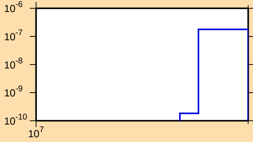
\sigma vs. E for ^{125}\text{Sb}(n,nt)
