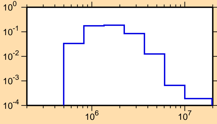
\sigma vs. E for ^{125}\text{Sb}(n,n_2)
