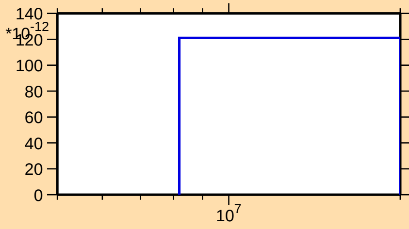
\sigma vs. E for ^{125}\text{Sb}(n,2np)
