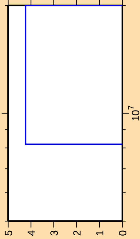
\Delta\sigma/\sigma vs. E for ^{125}\text{Sb}(n,2n)
