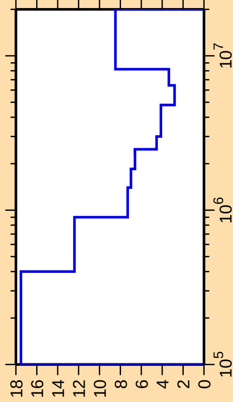
\Delta\sigma/\sigma vs. E for ^{125}\text{Sb}(n,\text{inel.})
