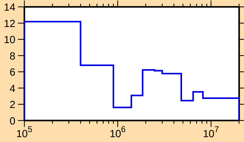
\Delta\sigma/\sigma vs. E for ^{125}\text{Sb}(n,\text{el.})
