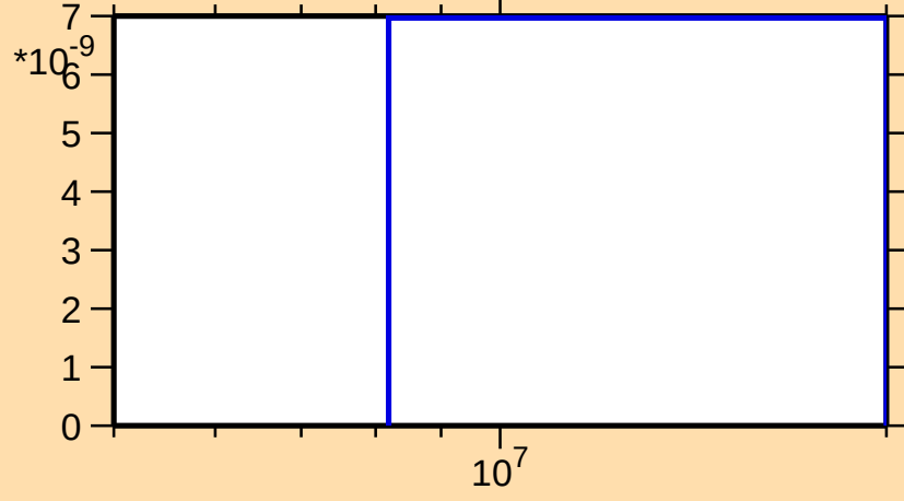
\sigma vs. E for ^{125}\text{Sb}(n,\text{nd})
