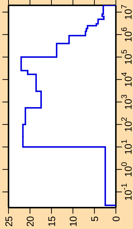
\Delta\sigma/\sigma vs. E for ^{125}\text{Sb}(n,\text{nonel.})
