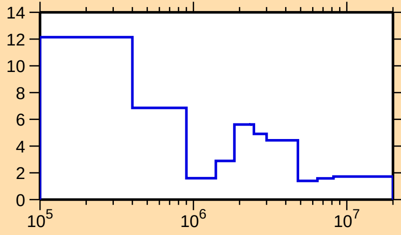
\Delta\sigma/\sigma vs. E for ^{125}\text{Sb}(n,\text{tot.})
