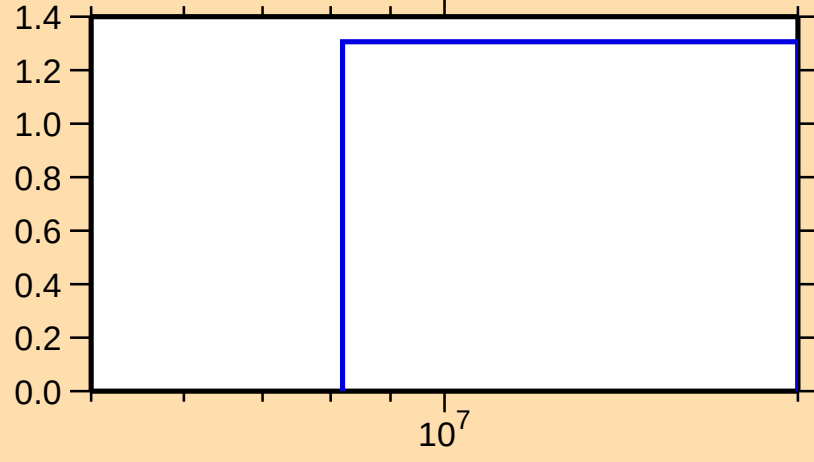
\sigma vs. E for ^{125}\text{Sb}(n,2n)
