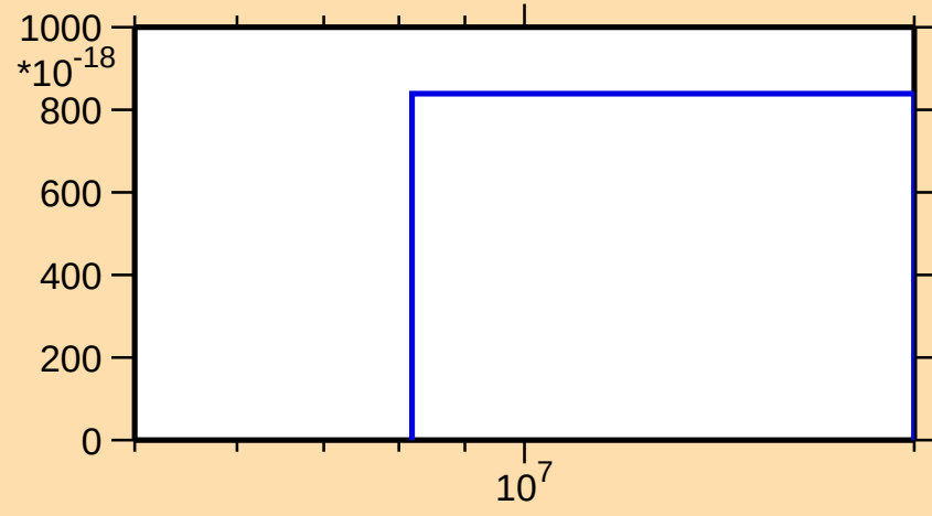
\sigma vs. E for ^{125}\text{Sb}(n,2n\alpha)
