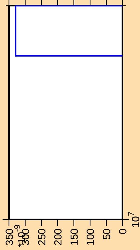
\Delta\sigma/\sigma vs. E for ^{126}\text{Sb} (mt 11)
