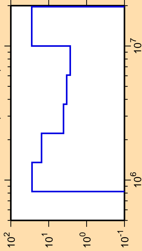
\Delta\sigma/\sigma vs. E for ^{126}\text{Sb}(n, ncont.)
