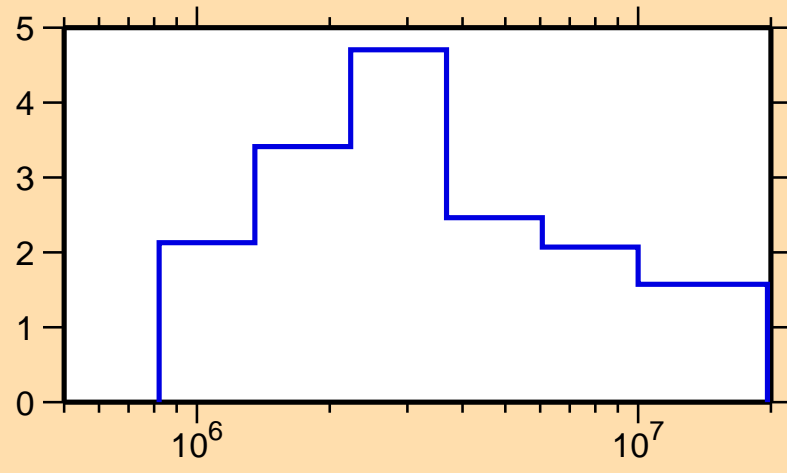
\Delta\sigma/\sigma vs. E for ^{126}\text{Sb}(n, tot.)
