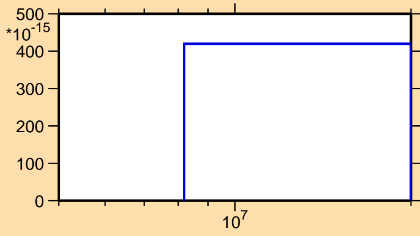
\sigma vs. E for ^{126}\text{Sb}(n,2n\alpha)
