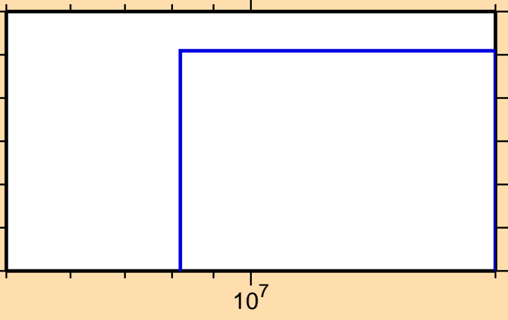
\sigma vs. E for ^{126}\text{Sb}(n,n\alpha)
