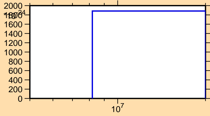
\sigma vs. E for ^{126}\text{Sb}(\text{mt } 11)
