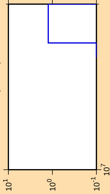
\Delta\sigma/\sigma vs. E for ^{126}\text{Sb}(n,\text{He3})
