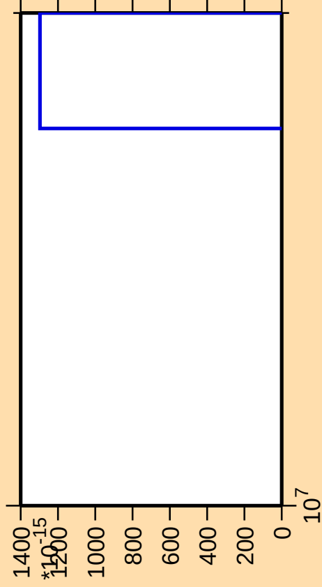
\Delta\sigma/\sigma vs. E for ^{126}\text{Sb}(\text{mt } 11)
