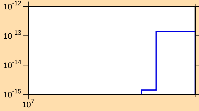
\sigma vs. E for ^{126}\text{Sb}(n,\text{He3})
