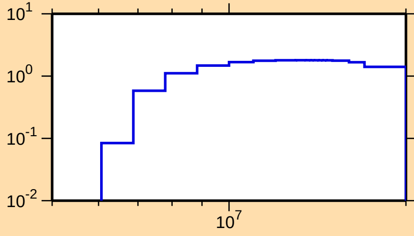
\sigma vs. E for ^{126}\text{Sb}(n,2n)
