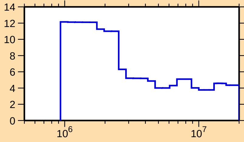
\Delta\sigma/\sigma vs. E for ^{126}\text{Sb}(n,n\text{oncl.})
