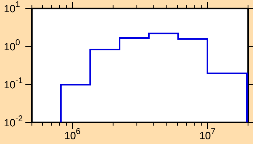
\sigma vs. E for ^{126}\text{Sb}(n,n\text{cont.})
