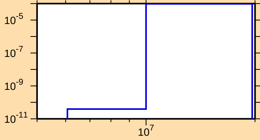
\sigma vs. E for ^{126}\text{Sb}(n,t)
