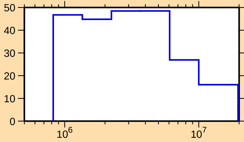
\Delta\sigma/\sigma vs. E for ^{126}\text{Sb}(n,\gamma)
