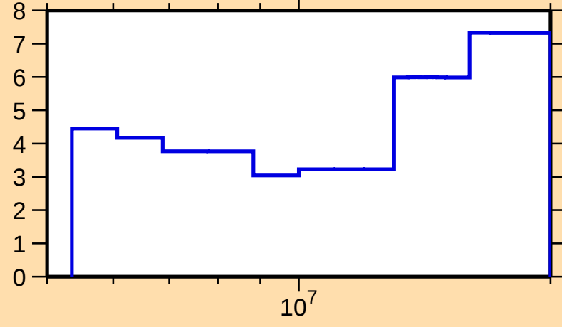
\Delta\sigma/\sigma vs. E for ^{130}\text{Sb}(n,\text{tot.})
