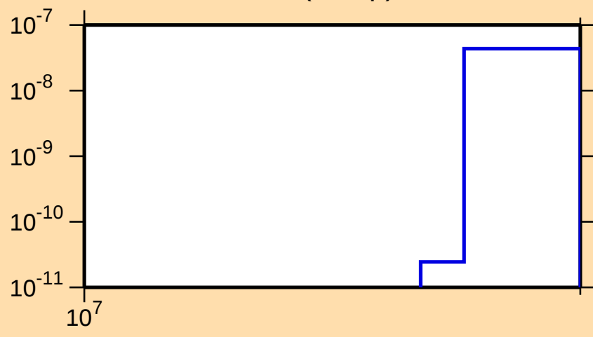
\sigma vs. E for ^{130}\text{Sb}(n,2np)
