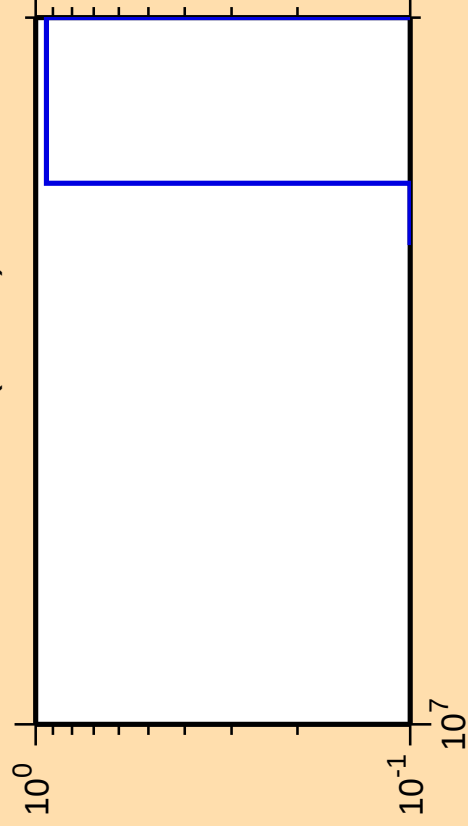
\Delta\sigma/\sigma vs. E for ^{130}\text{Sb}(n,2n\alpha)
