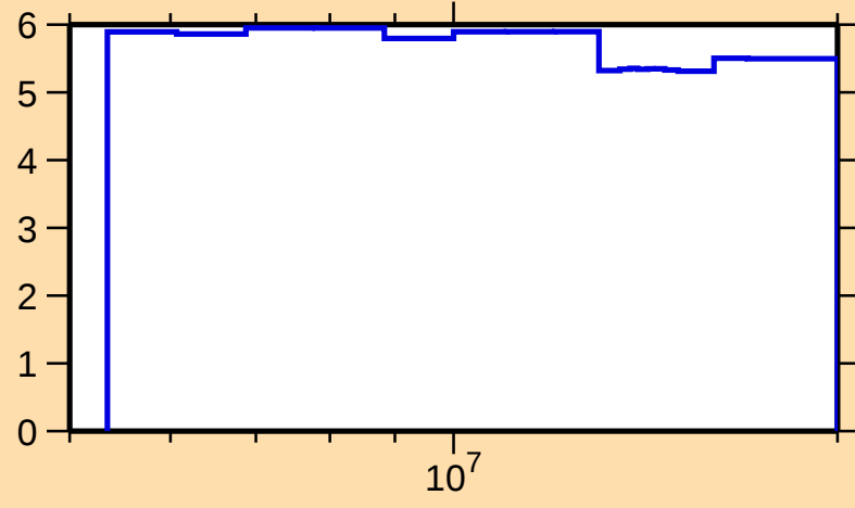
\Delta\sigma/\sigma vs. E for ^{130}\text{Sb}(n,\text{nonel.})
