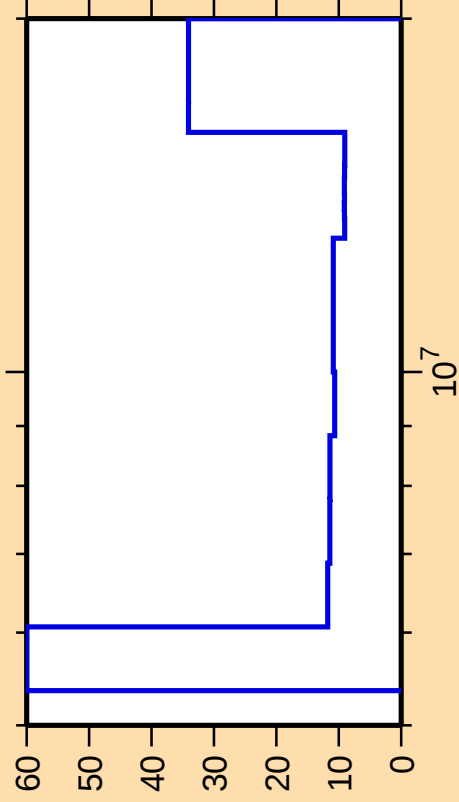
\Delta\sigma/\sigma vs. E for ^{130}\text{Sb}(n,2n)
