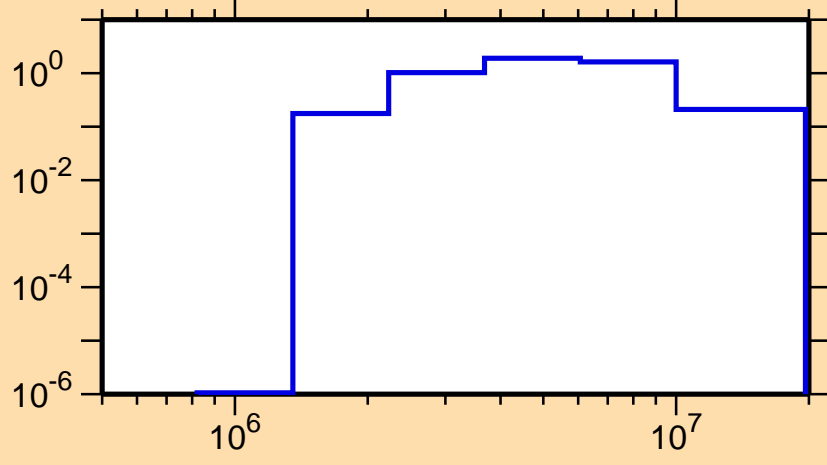
\sigma vs. E for ^{130}\text{Sb}(n,n\text{cont.})
