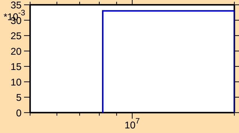
\sigma vs. E for ^{130}\text{Sb}(n,3n)
