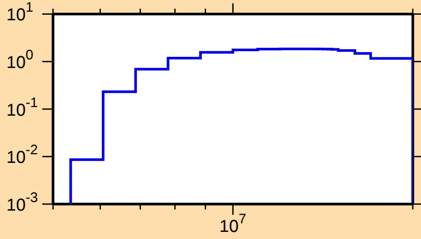
\sigma vs. E for ^{130}\text{Sb}(n,2n)
