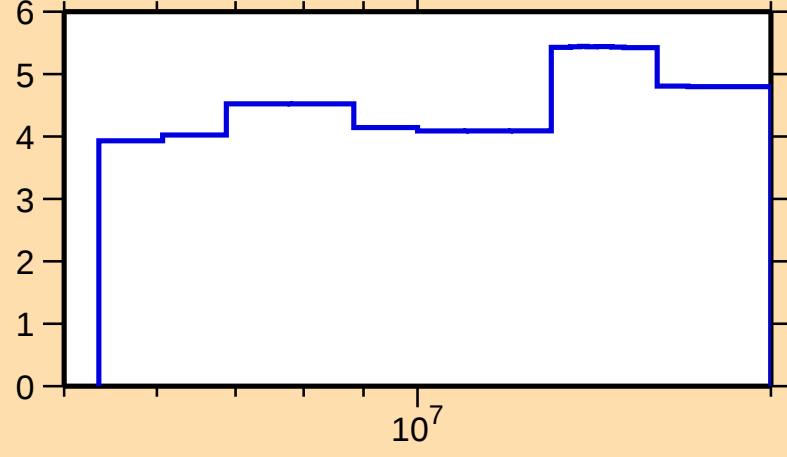
\Delta\sigma/\sigma vs. E for ^{130}\text{Sb}(n,\text{nonel.})
