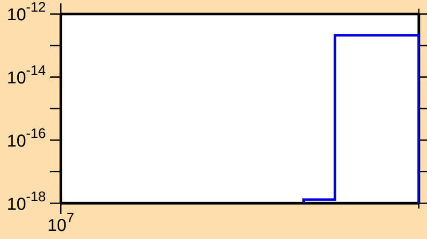
\sigma vs. E for ^{130}\text{Sb}(n,2n\alpha)
