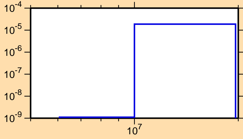
\sigma vs. E for ^{130}\text{Sb}(n,\alpha)
