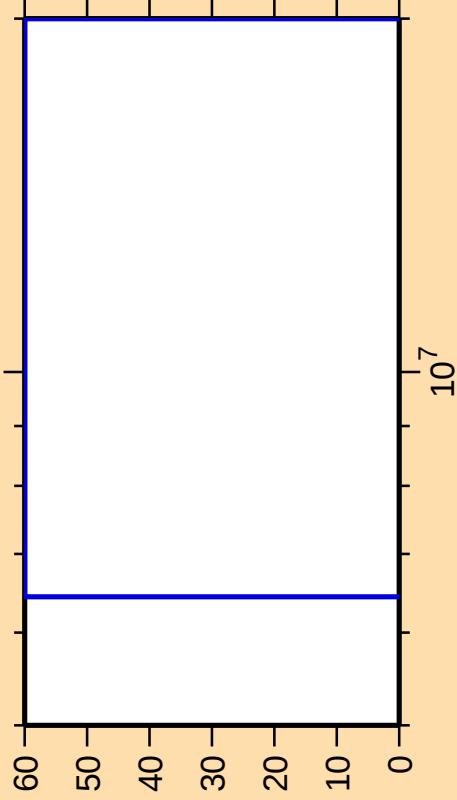
\Delta\sigma/\sigma vs. E for ^{130}\text{Sb}(n,\alpha)
