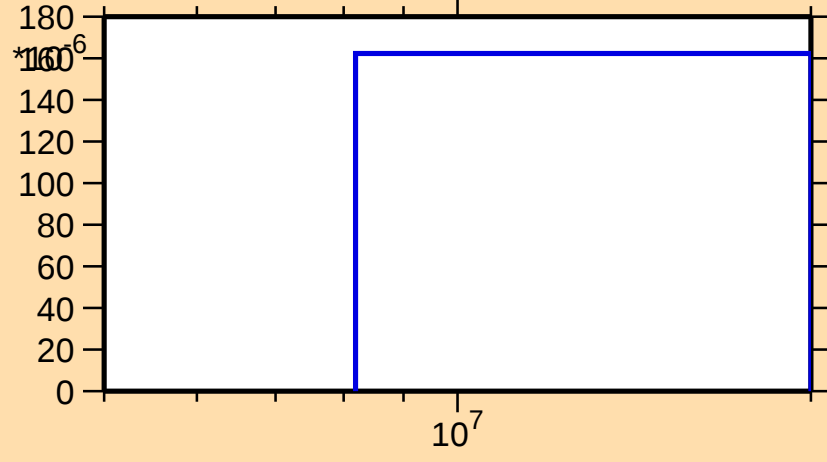
\sigma vs. E for ^{130}\text{Sb}(n,np)
