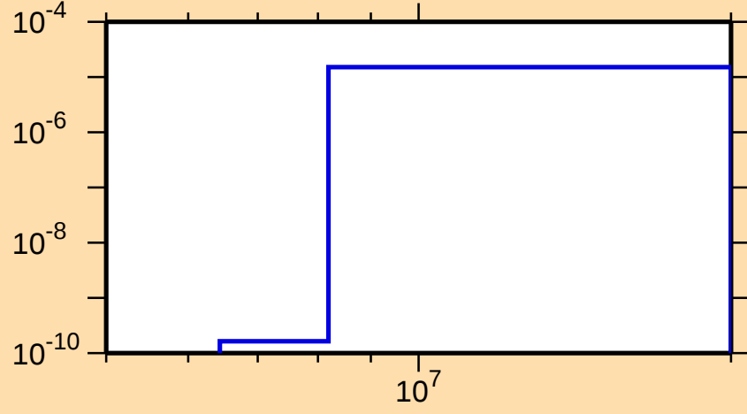
\sigma vs. E for ^{130}\text{Sb}(n,\alpha)
