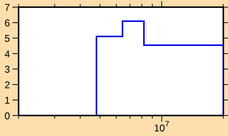
\Delta\sigma/\sigma vs. E for ^{130}\text{Sb}(n,\text{el.})
