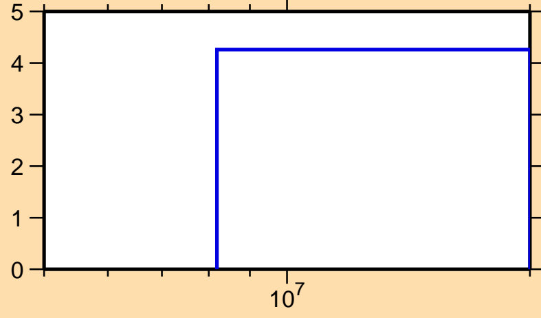
\Delta\sigma/\sigma vs. E for ^{131}\text{Sb}(n,\text{el.})
