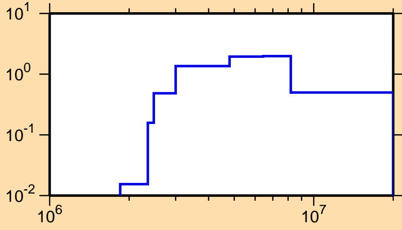
\sigma vs. E for ^{131}\text{Sb}(n,n\text{cont.})
