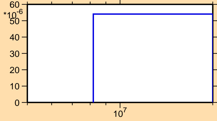
\sigma vs. E for ^{131}\text{Sb}(n,np)
