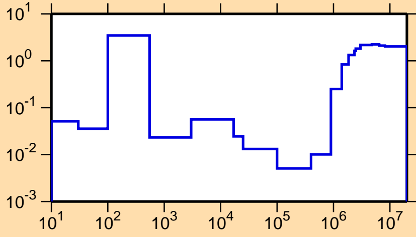
\sigma vs. E for ^{131}\text{Sb}(n,\text{nonel.})
