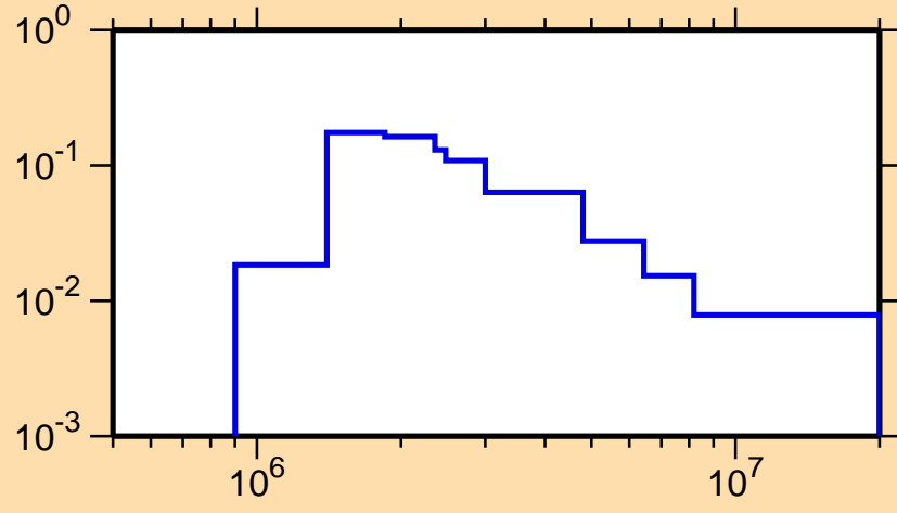
\sigma vs. E for ^{131}\text{Sb}(n,n_4)
