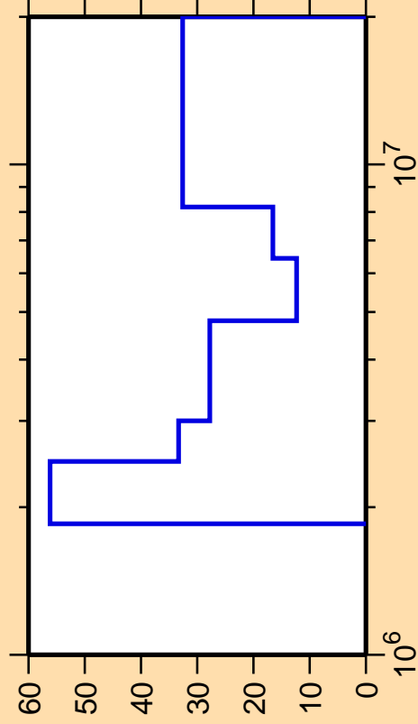
\Delta\sigma/\sigma vs. E for ^{131}\text{Sb}(n,n\text{cont.})
