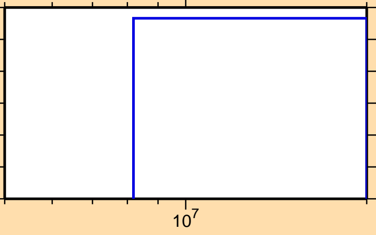
\sigma vs. E for ^{131}\text{Sb}(n,n\alpha)
