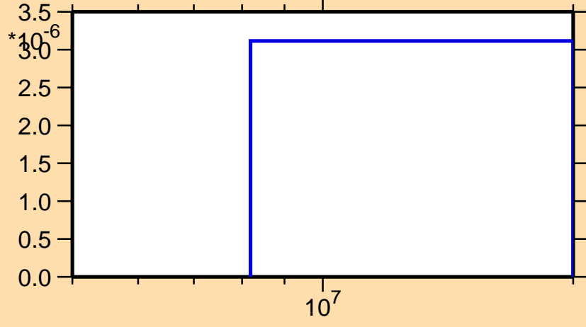
\sigma vs. E for ^{131}\text{Sb}(n,t)
